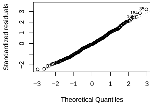
Q-Q Residuals
