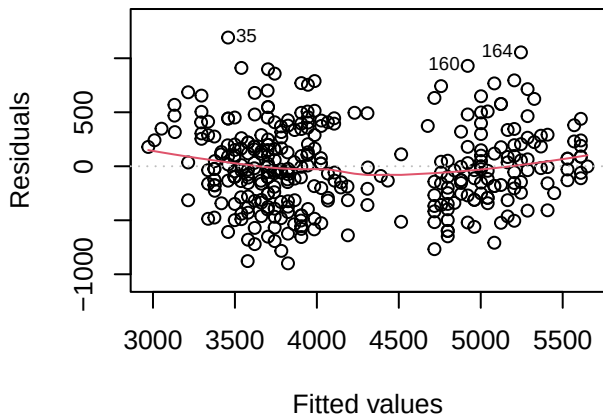
Residuals vs Fitted
