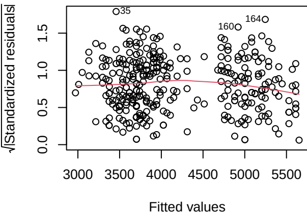
Scale-Location
