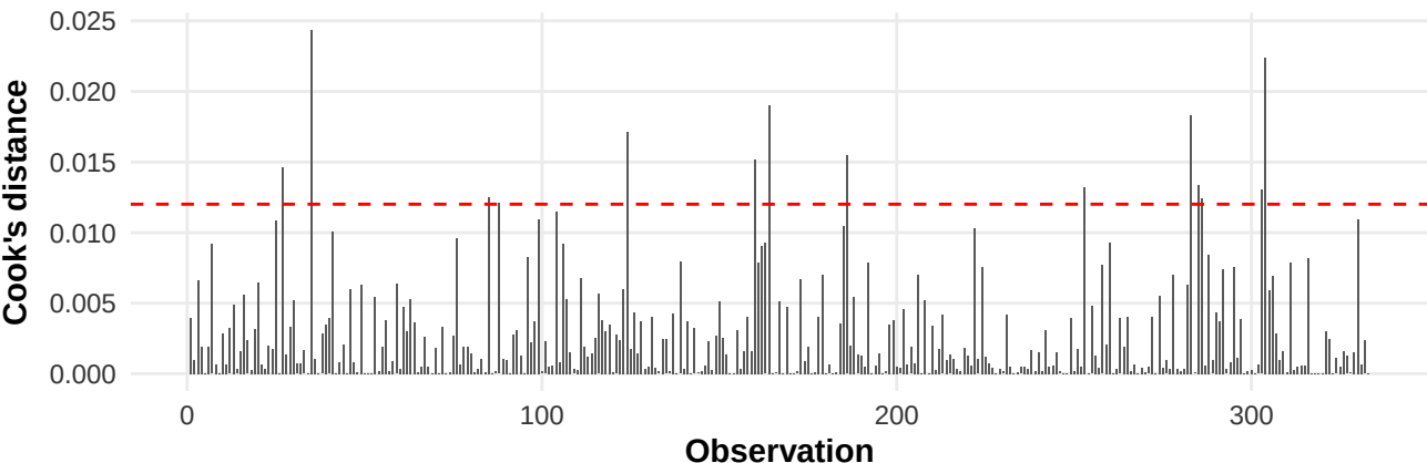
C. Cook's distance
