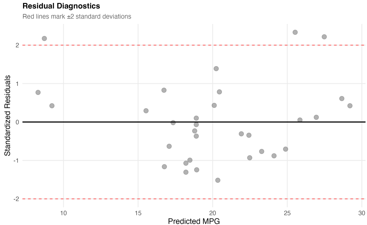
Figure 7: Residual diagnostic plot showing standardized residuals vs fitted values. The red dashed lines mark \pm 2 standard deviations. A good model should show residuals randomly scattered around zero with no patterns. We have a few potential outliers but overall the fit looks reasonable.
