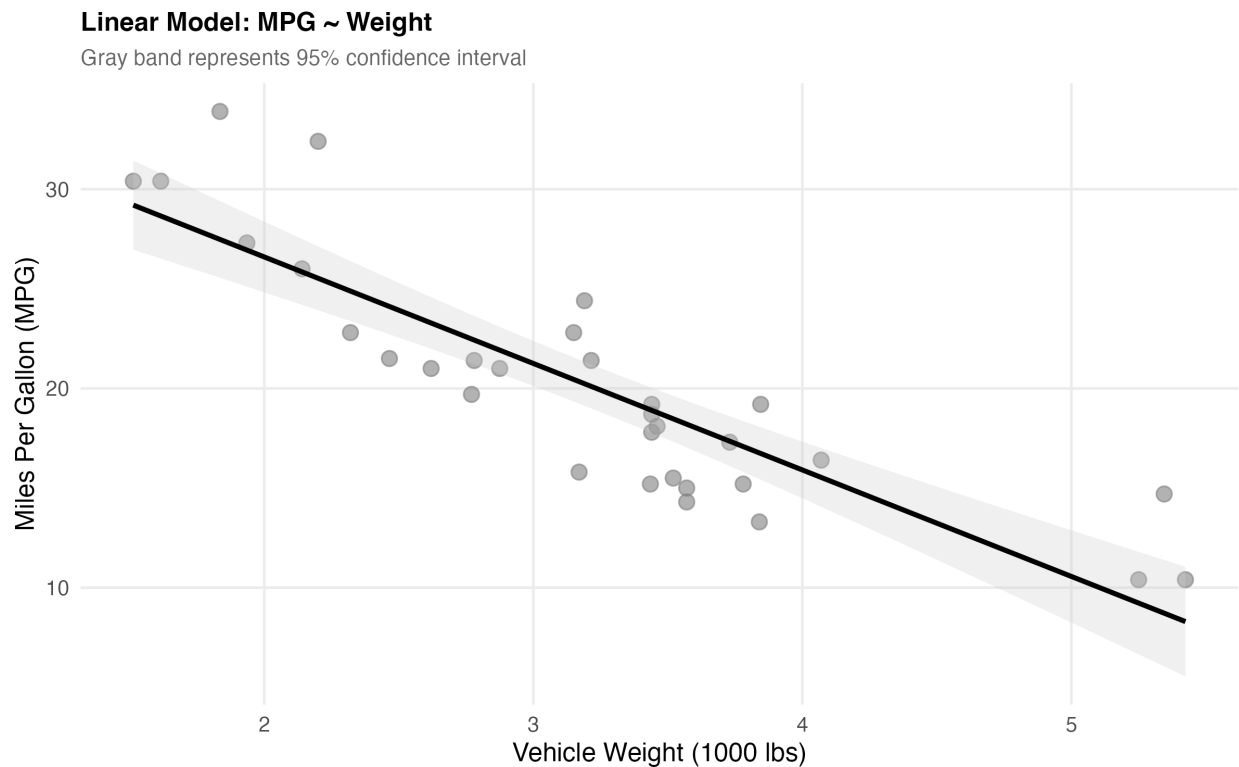
Figure 6: Linear regression fit showing the relationship between vehicle weight and fuel efficiency. The gray band represents the 95% confidence interval around the fitted line. The fit is quite good, explaining 75% of the variance in MPG.
