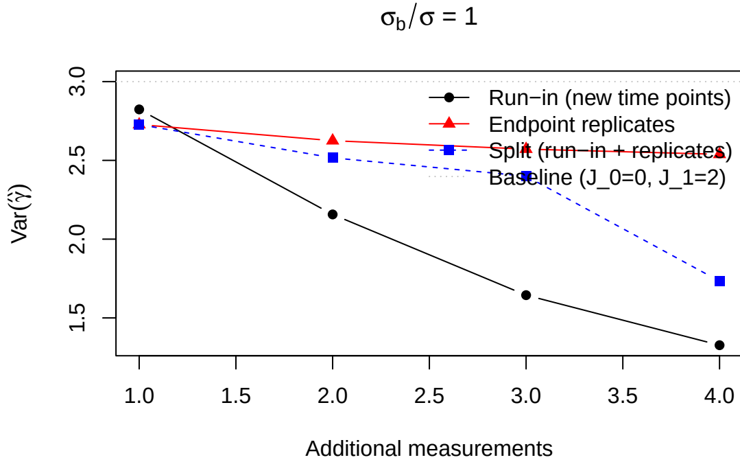
Figure 1: (#fig:rep_vs_runin) Variance as a function of additional measurements allocated either to run-in (new time points) or endpoint replication (same time point). Baseline: J_0 = 0 , J_1 = 2 , \sigma^2 = 1 , \sigma_b^2 = 1 .
