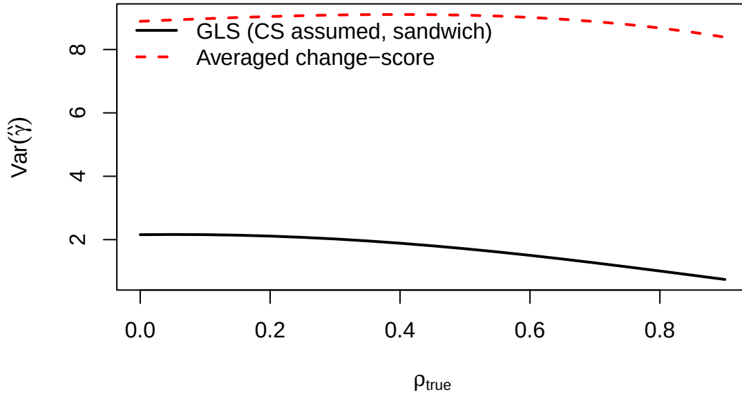
Figure 2: (#fig:misspec_R)Effect of analyzing under compound symmetry when the true correlation is AR(1). Sandwich variance of GLS (solid) vs averaged change-score on the \gamma scale (dashed) as a function of \rho . The averaged estimator's definition does not use the assumed correlation, but its variance varies with the true R ; GLS remains at least fourfold more efficient at every \rho .
