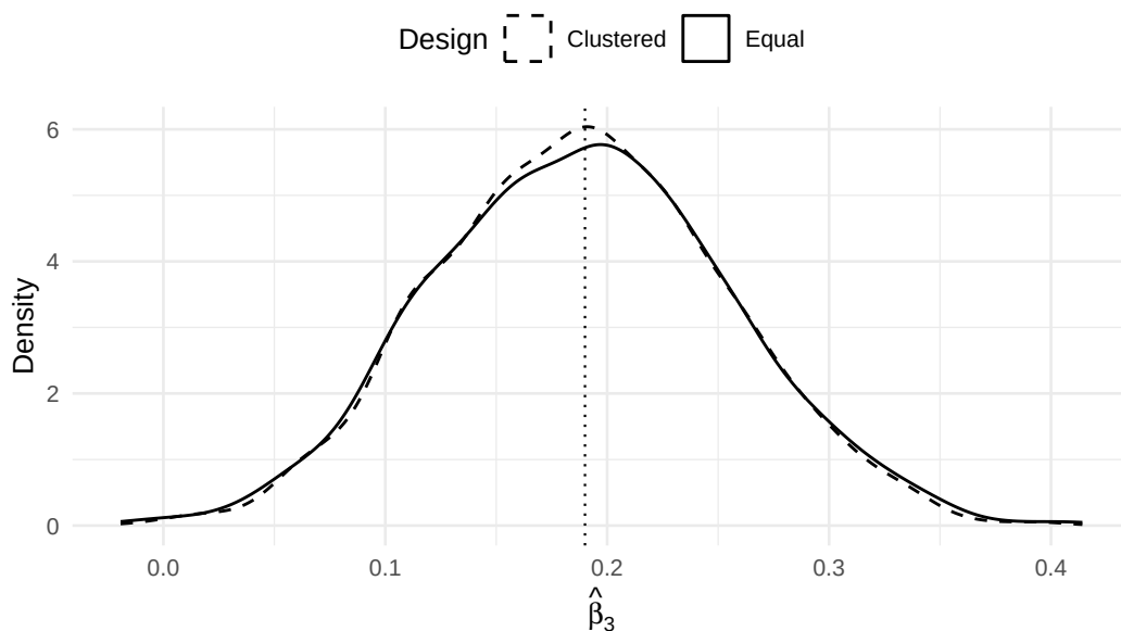
Figure 2: Sampling distribution of the treatment-by-time interaction estimate under each design.
