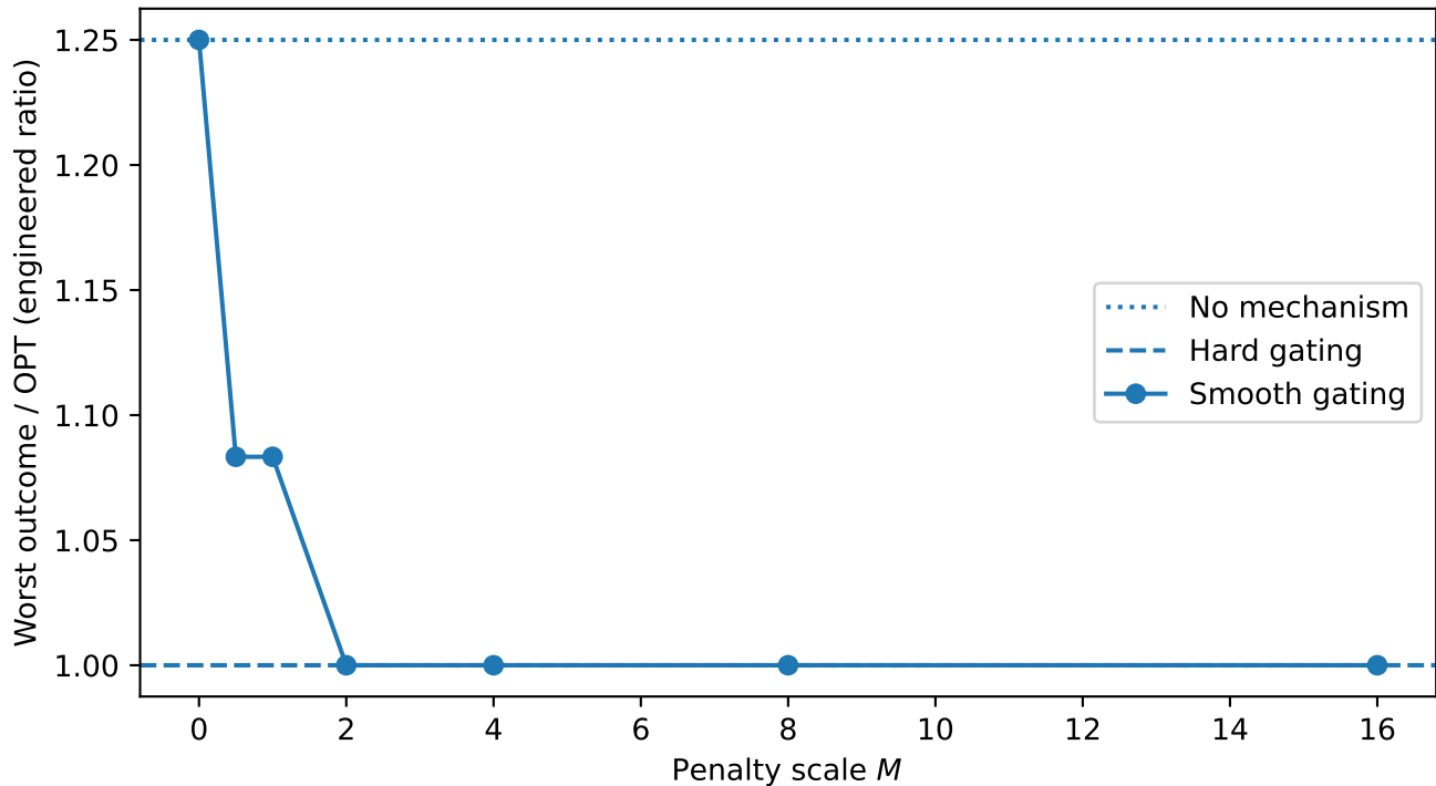
Smooth penalties vs hard gating (Pigou-style atomic routing)
