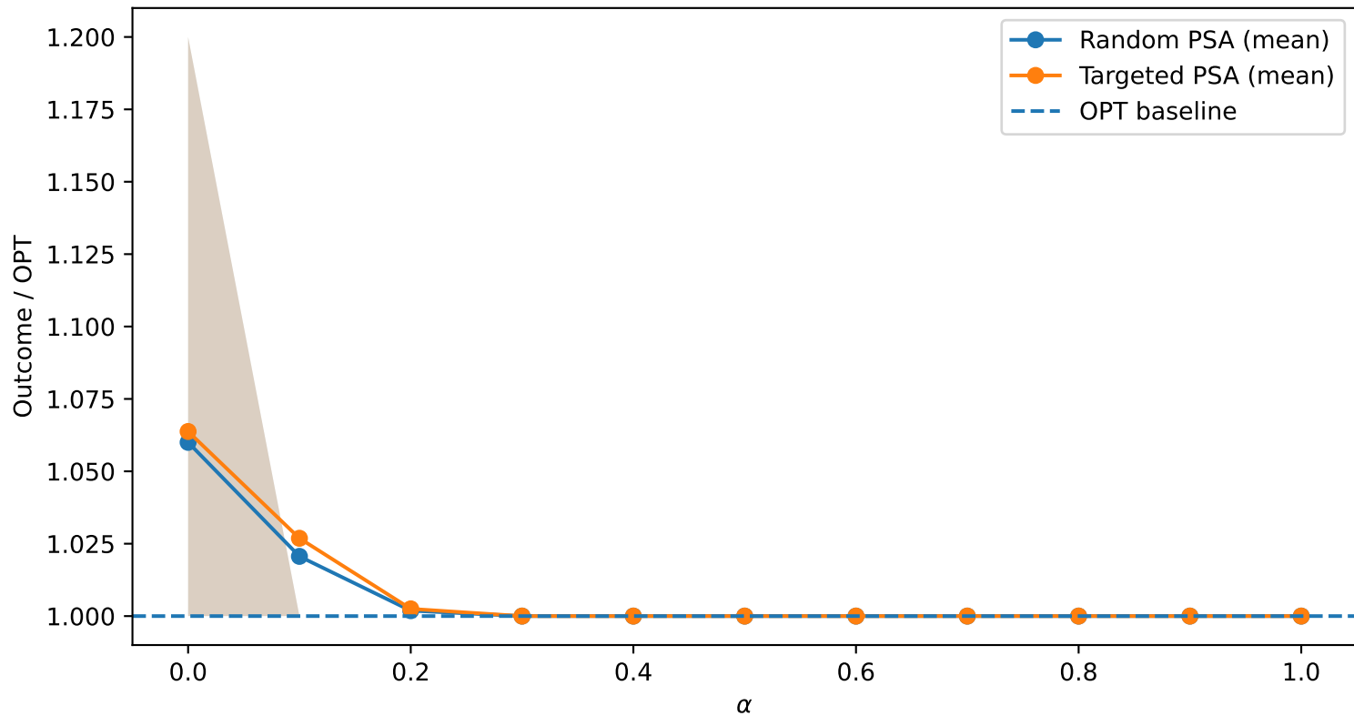
Cost-sharing (threshold instance): PSA vs \alpha (bands = IQR over PSA trials)
