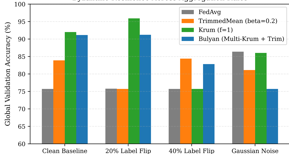
Byzantine Resilience Across Aggregation Rules
