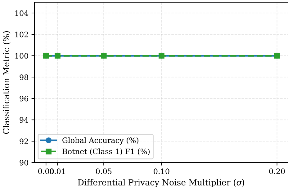
Privacy-Utility Trade-off Curve (DP-SGD Bounds)
