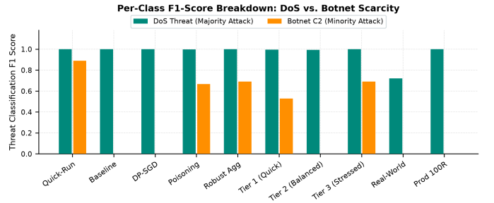
Fig. 12. Per-class F1-score breakdown across benchmark configurations. DoS (teal) vs. Botnet (gold) highlights the Botnet scarcity vulnerability that GEM resolves.
