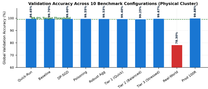
Fig. 11. Validation accuracy across 10 benchmark configurations on the physical Proxmox VE cluster. Nine configurations exceed the 99.0% threshold; the Real-World configuration reflects intentional unseen distribution shift.
