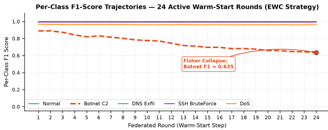
Fig. 6. Per-class F1-score trajectories over 24 active rounds. Botnet (Class 1) exhibits monotonic decline from 0.89 to 0.63 while all other classes remain above 0.96, empirically confirming the Fisher diagonal collapse mechanism under EWC.
