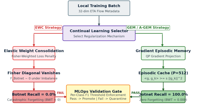
Fig. 2. Continual learning strategy decision flow. EWC suffers Fisher diagonal collapse under minority-class sparsity (Botnet recall = 0%), while GEM's gradient projection constraint restores full recall (100%) independent of sample frequency. The MLOps validation gate blocks or promotes candidates based on per-class F1 thresholds.
