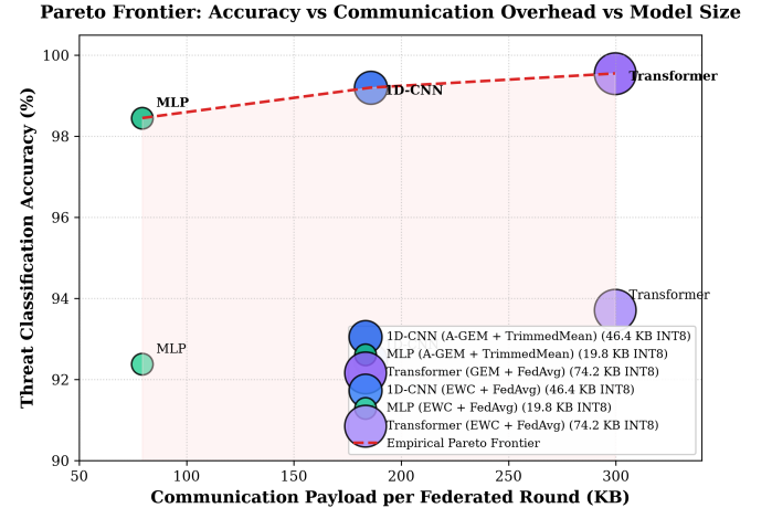
Fig. 13. Empirical Pareto Frontier: Threat classification accuracy (%) versus communication payload per round (KB) and INT8 quantized footprint across evaluated backbones.
