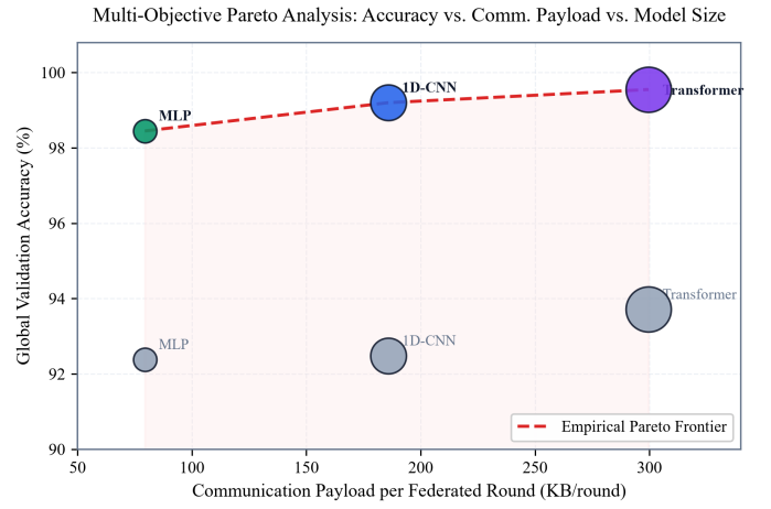
Fig. 14. Empirical Pareto Frontier: Threat classification accuracy (%) versus communication payload per round (KB) and INT8 quantized footprint across evaluated backbones.
