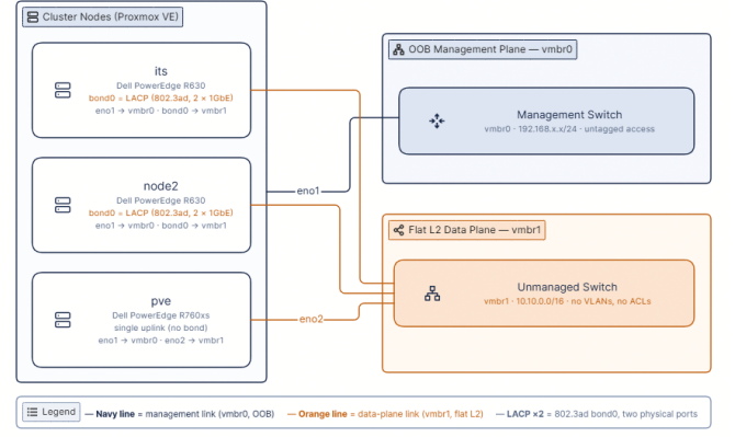
Fig. 1. FL-CL system architecture deployed on a 3-node Proxmox VE cluster. Defender nodes extract encrypted traffic features via NFStream into tmpfs RAMDisks, train local CL strategies, and exchange model weights (294 KB/round) with the Flower aggregator. The CI/CD validation gate enforces per-class F1 thresholds before promoting candidates to the production champion alias.
