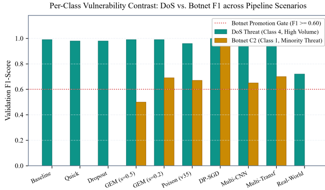
Fig. 13. Per-class F1-score breakdown across benchmark configurations. DoS (teal) vs. Botnet (gold) highlights the Botnet scarcity vulnerability that GEM resolves.
