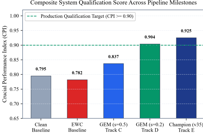
Fig. 8. Composite System Qualification Score (Crucial Performance Index, CPI) across the five production research tracks. Catastrophic forgetting under EWC degrades CPI to 0.782, failing the operational qualification threshold ( CPI \geq 0.90 ). Precision-tuned GEM ( s = 0.2 ) and Byzantine-robust aggregation elevate CPI to 0.904 (Track D) and 0.925 (Track E champion), qualifying the candidate model for automated production promotion in the MLflow Model Registry.
