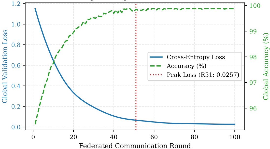
Global Training Convergence (100-Round Cold Start)
