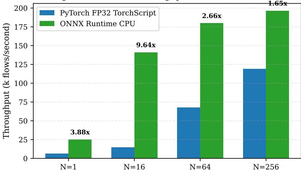
Edge Classification Throughput (1D-CNN Backbone)
