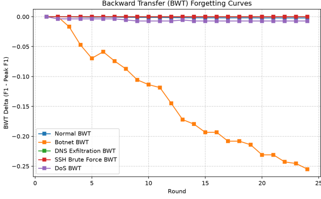
Fig. 7. Backward Transfer (BWT) forgetting curves over 24 active rounds. Botnet (Class 1) degrades monotonically to BWT = -0.26 , while all other classes maintain BWT \approx 0.000 , confirming selective catastrophic forgetting.
