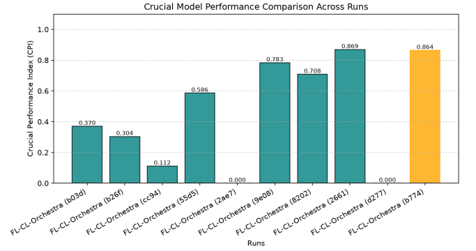
Fig. 13. Crucial Performance Index (CPI) comparison across FL-CL orchestration runs. The v35 champion (CPI = 0.864) achieved fully automated promotion through all five per-class F1 gates.
