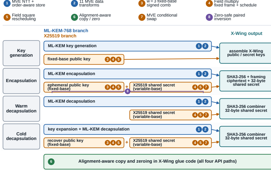
Fig. 1. X-Wing data flow and scope of the eight retained optimizations. Numbered badges refer to Table 1. The fixed-base comb is absent from warm decapsulation, MVE cswap is confined to variable-base ladders, and zero-safe paired inversion links the two X25519 outputs only during encapsulation. Alignment-aware copy and zeroing span all four API paths.
