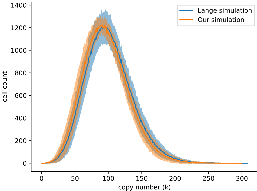
ecDNA copy number distributions
