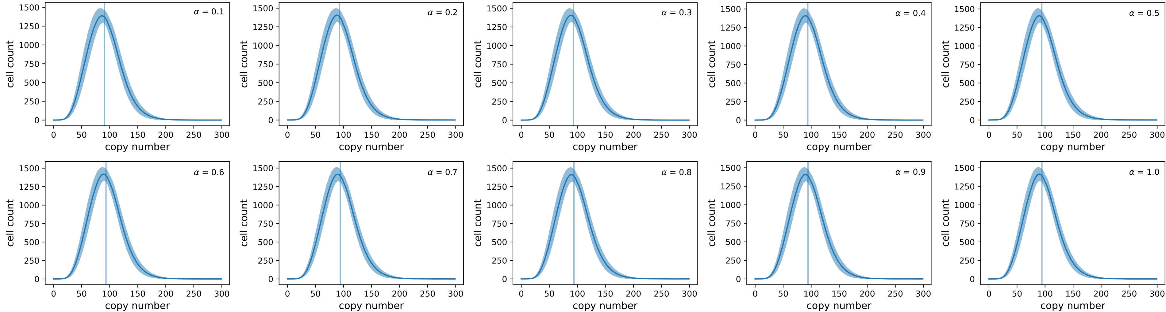
Copy number distributions for varying \alpha , k_0 = 50 , k^* = 100
