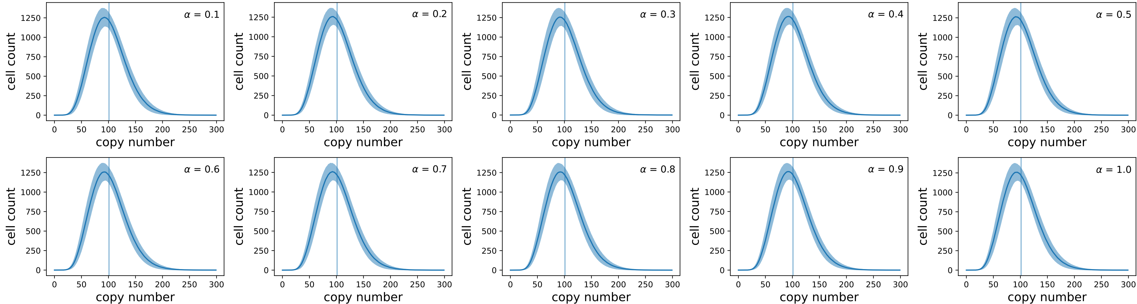
Copy number distributions for varying \alpha , k_0 = 100 , k^* = 50
