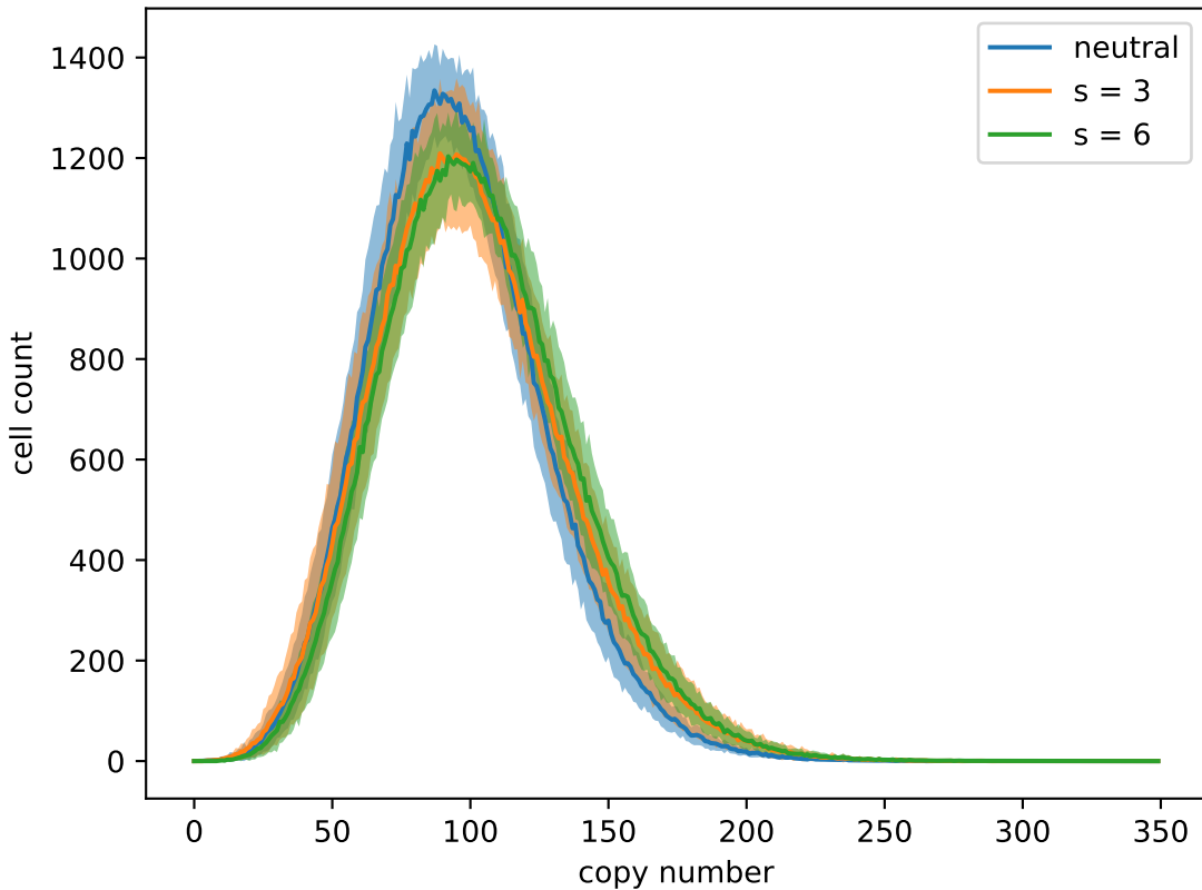
Copy number distributions for Lange model of selection
