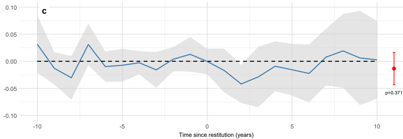
Log(EVI) - Plantation Forest
