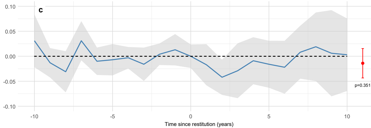
Log(EVI) - Plantation Forest
