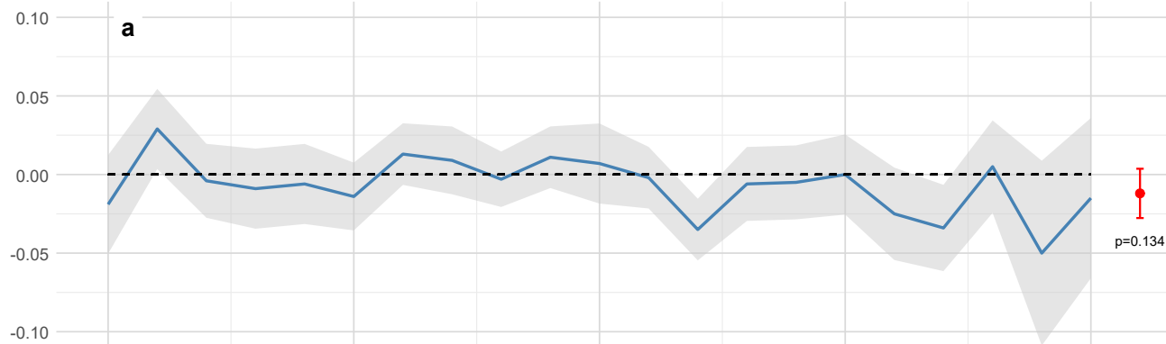
Log(EVI) - Natural Forest
