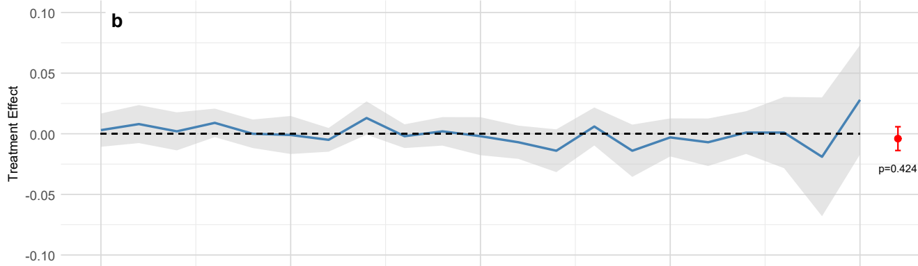
Log(EVI) - Plantation Forest
