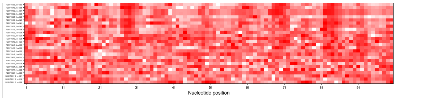
Continuous SGNM-predicted reactivity (per-row normalized), sorted by correlation to the reference-model profile.
