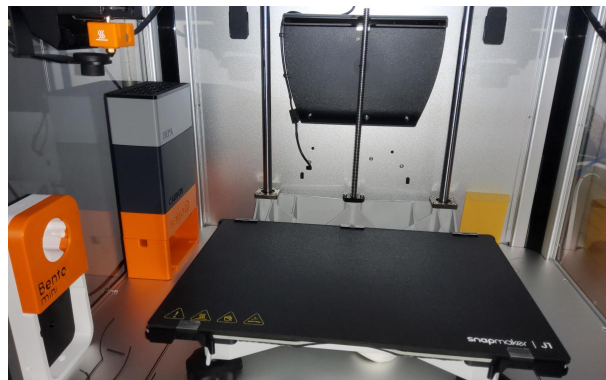
BentoBoxV2 in Snapmaker J1.
