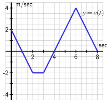
Figure 1: The graph of the velocity function, v(t) .
