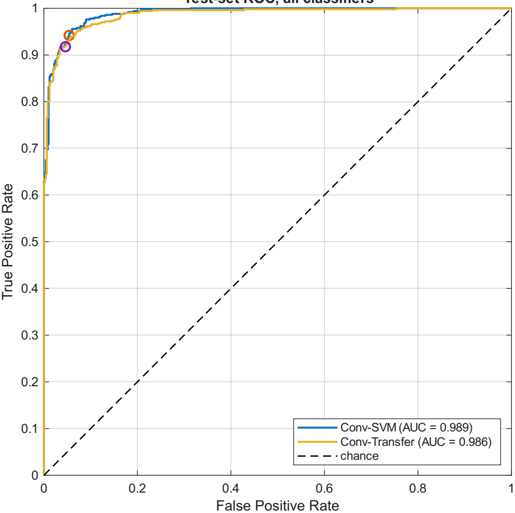
Test-set ROC, all classifiers
