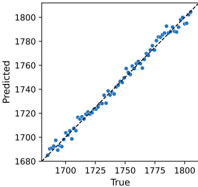
Resonance \lambda (nm) R^2 = 0.991
