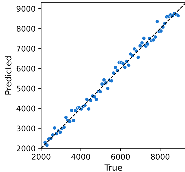
Sensitivity (nm/RIU) R^2 = 0.990
