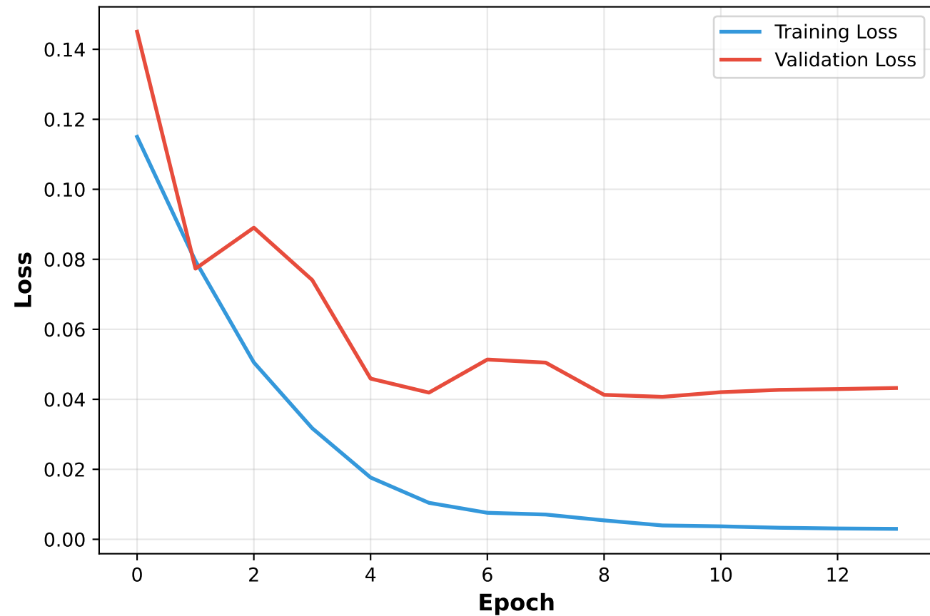
LSTM - Loss
