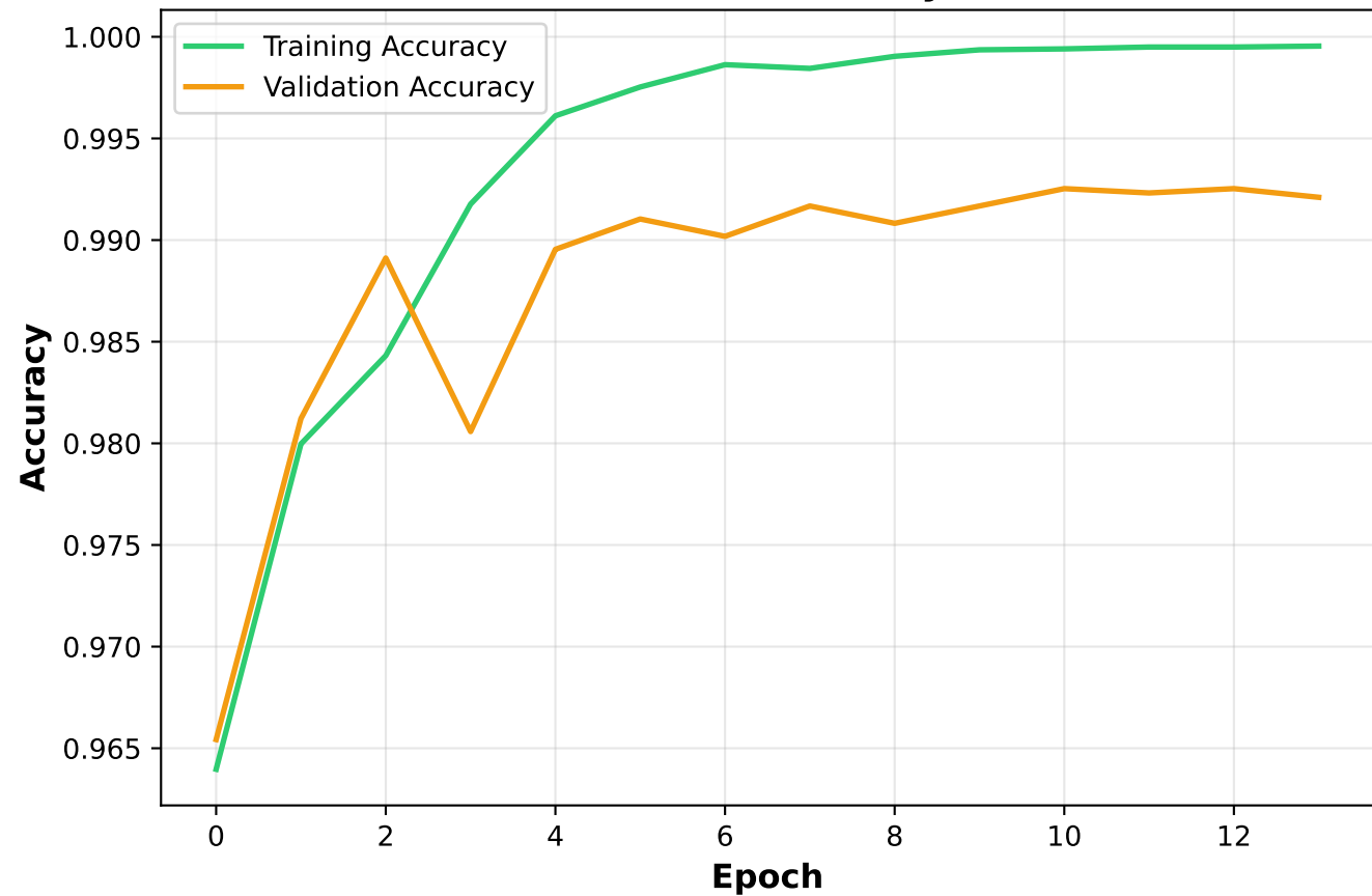
LSTM - Accuracy
