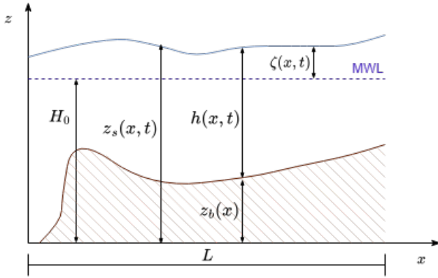
Fig. 1: Schematic longitudinal view of the 1D shallow-water configuration, showing the bed elevation z_b(x) , the free-surface level z_s(x, t) , the surface elevation relative to the Mean Water Level (MWL) \zeta(x, t) , the water depth h(x, t) , the reference still-water depth H_0 , and the domain length L .
