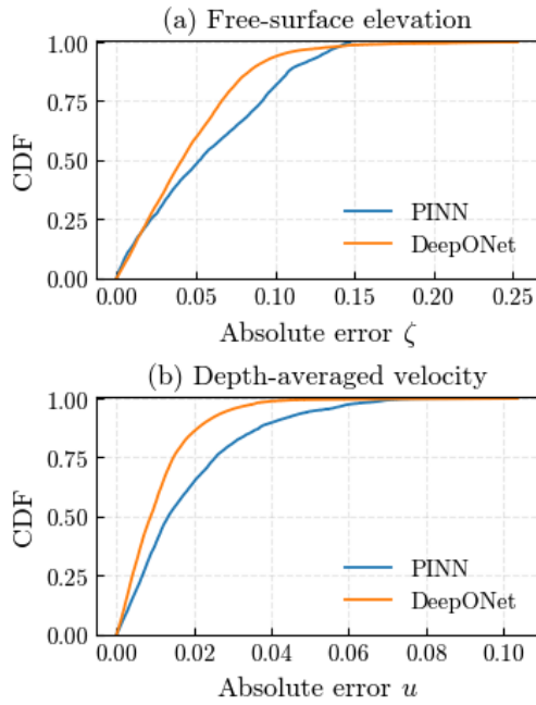
Fig. 9: Empirical Cumulative Distribution Functions (CDFs) of the pointwise absolute errors produced by the PINN and DeepONet surrogate models predicting the (a) free-surface elevation, and (b) depth-averaged velocity of the randomly generated unseen scenario.
