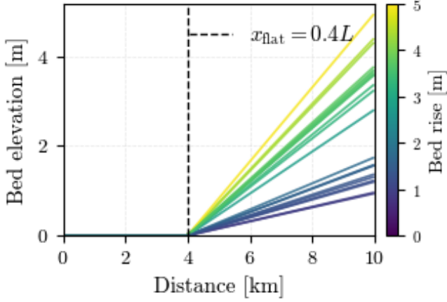
Fig. 4: Bathymetric profiles of the 20 independently generated training scenarios. In each one, the bed is flat on the horizontal axis until x_{\text{flat}} , where it increases linearly to a randomly sampled final bed elevation from the interval [1, 5] m at x = L . This variation allows both surrogate models to be trained across different physical configurations.
