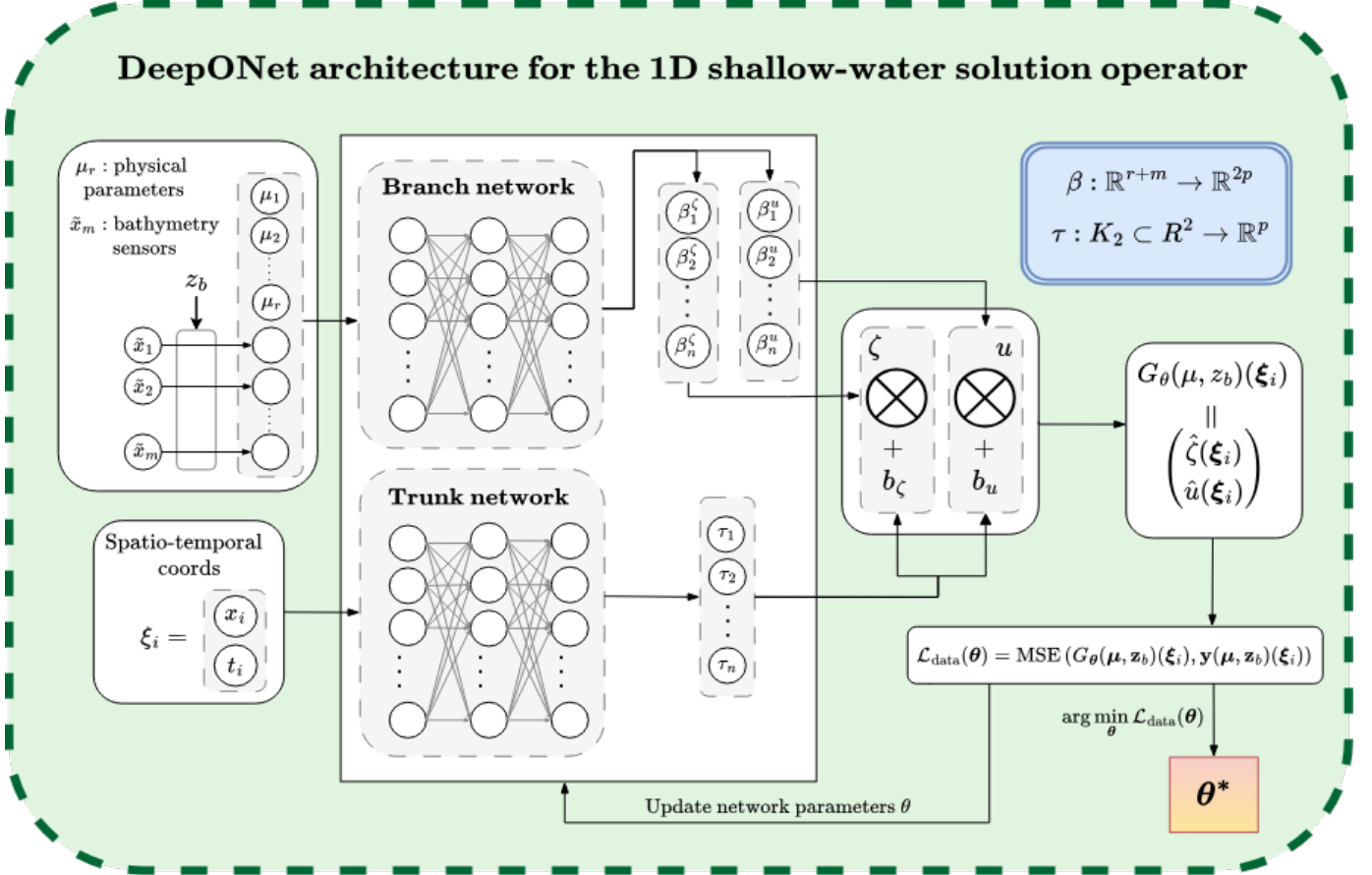
Fig. 3: DeepONet’s architecture and training workflow used for the surrogate modeling of the one-dimensional shallow-water equations used in this work. As explained before, this architecture consists of two neural networks, referred to as the branch and trunk networks. After setting up an initial configuration of the PDE, the branch network receives a finite-dimensional description of it, consisting of a vector of physical parameters \mu = (\mu_1, \dots, \mu_r) and the bathymetric profile z_b evaluated at m fixed sensor locations \{\tilde{x}_1, \dots, \tilde{x}_m\} . Note that the number of physical parameters can change depending on the problem setting. One may include wind speed, tidal amplitude and frequency, storm forcing parameters like wind direction, bottom-drag coefficients, etc.
