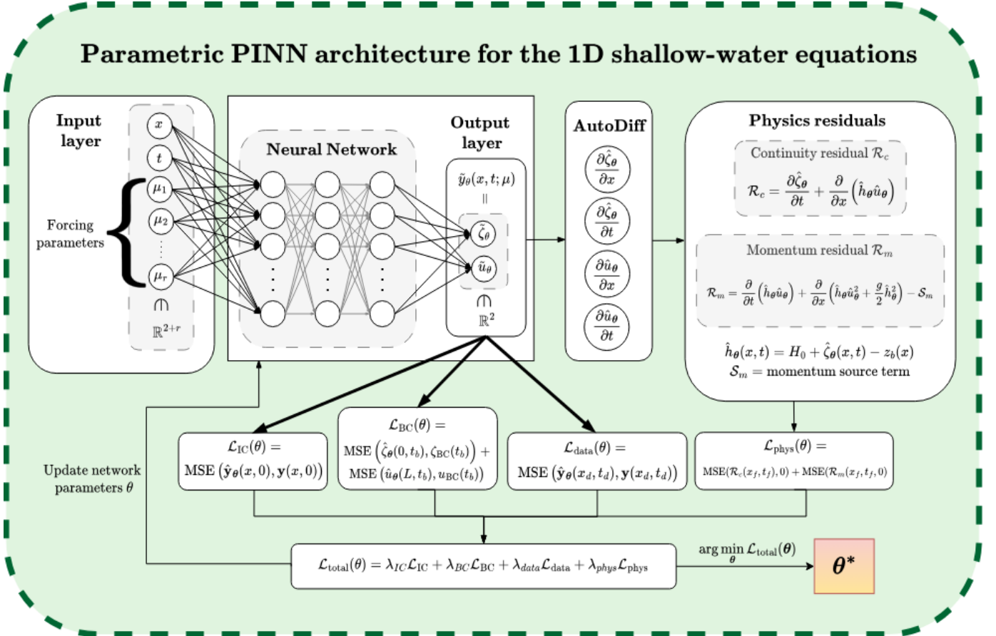
Fig. 2: Schematic showing the PINN architecture and training workflow used for the surrogate modeling of the parametric one-dimensional shallow-water equations considered in this work. A single feedforward neural network is employed, whose inputs are the spatio-temporal coordinates (x, t) and a physical-parameter vector denoted by \mu = (\mu_1, \dots, \mu_r) . This vector may include storm properties, wind conditions, etc. (conditions that change between training samples).
