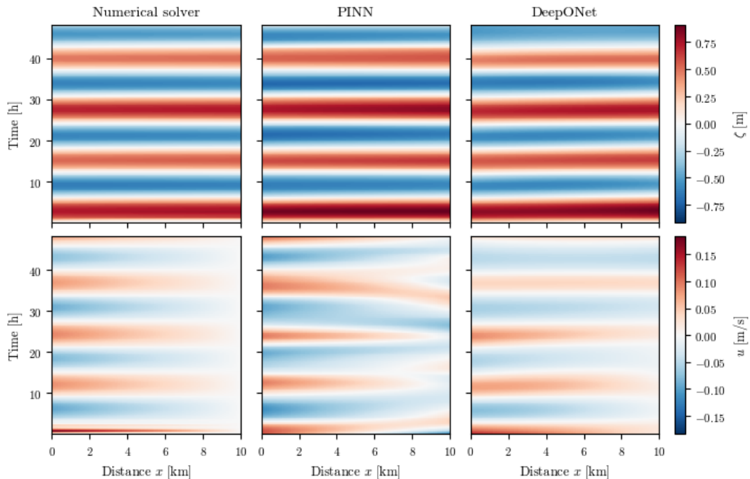
Fig. 8: Space-time heatmaps of the free-surface elevation (top row) and depth-averaged velocity (bottom row) for the unseen scenario. The columns show the numerical reference solution, PINN prediction, and DeepONet prediction, respectively.
