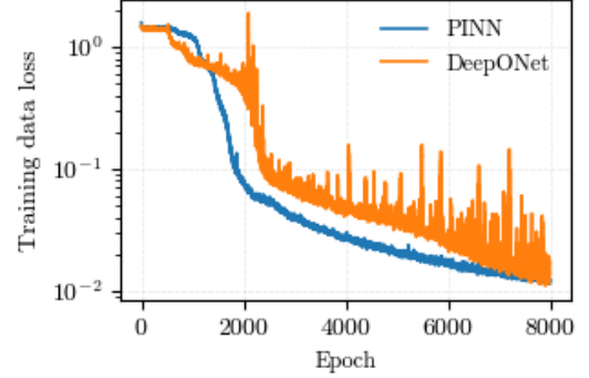
Fig. 7: Evolution of the supervised training-data loss of both the PINN and DeepONet surrogate models over the training epochs.
