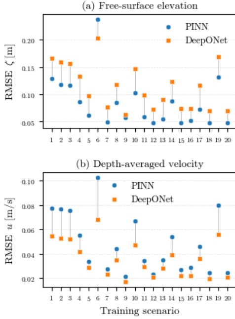
Fig. 5: Space-time final RMSE of the PINN and DeepONet predictions across the 20 training scenarios for (a) free-surface elevation and (b) depth-averaged velocity after the training process.
