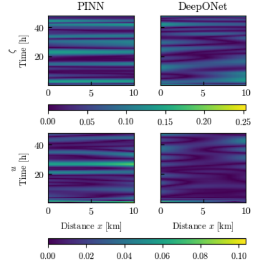
Fig. 6: Space-time absolute-error heatmap of both the predictions from the PINN and DeepONet models for the randomly generated unseen scenario whose forcing and bathymetric parameters lie within the ranges used for generating the training scenarios.
