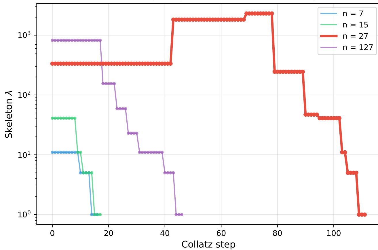
Skeleton trajectory: \lambda value at each Collatz step
