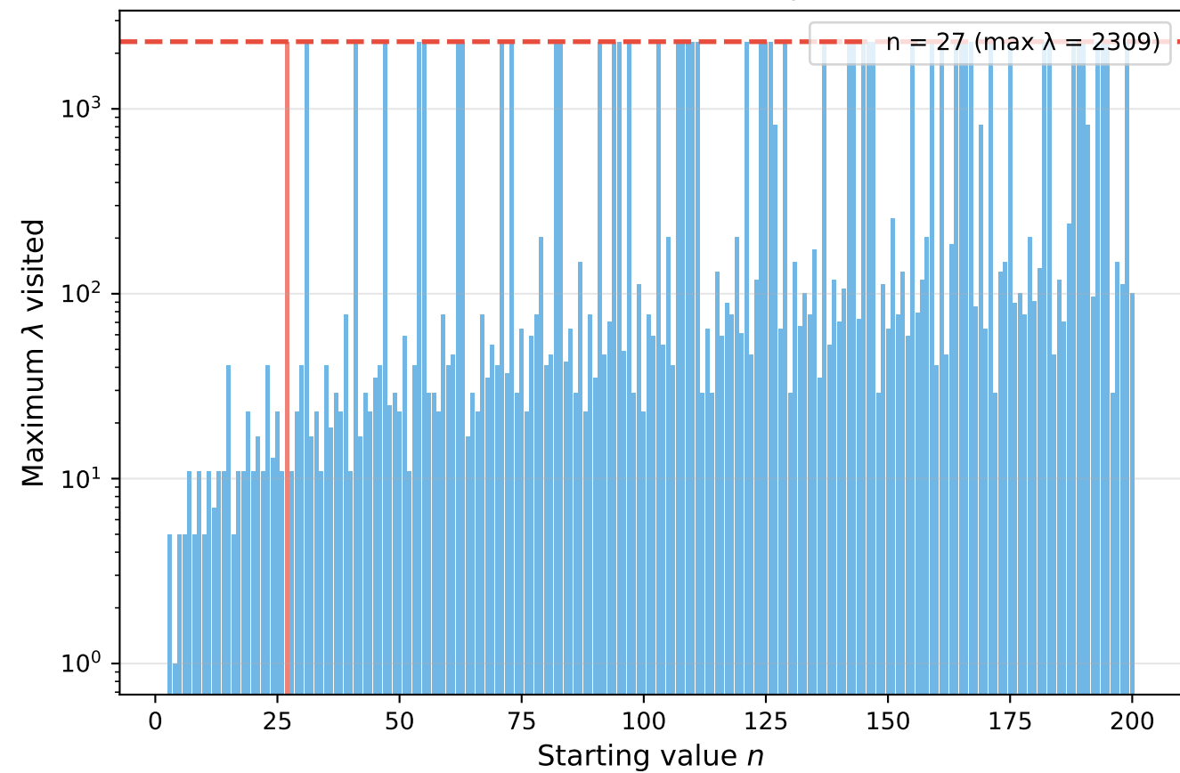
Maximum skeleton \lambda reached by each orbit
