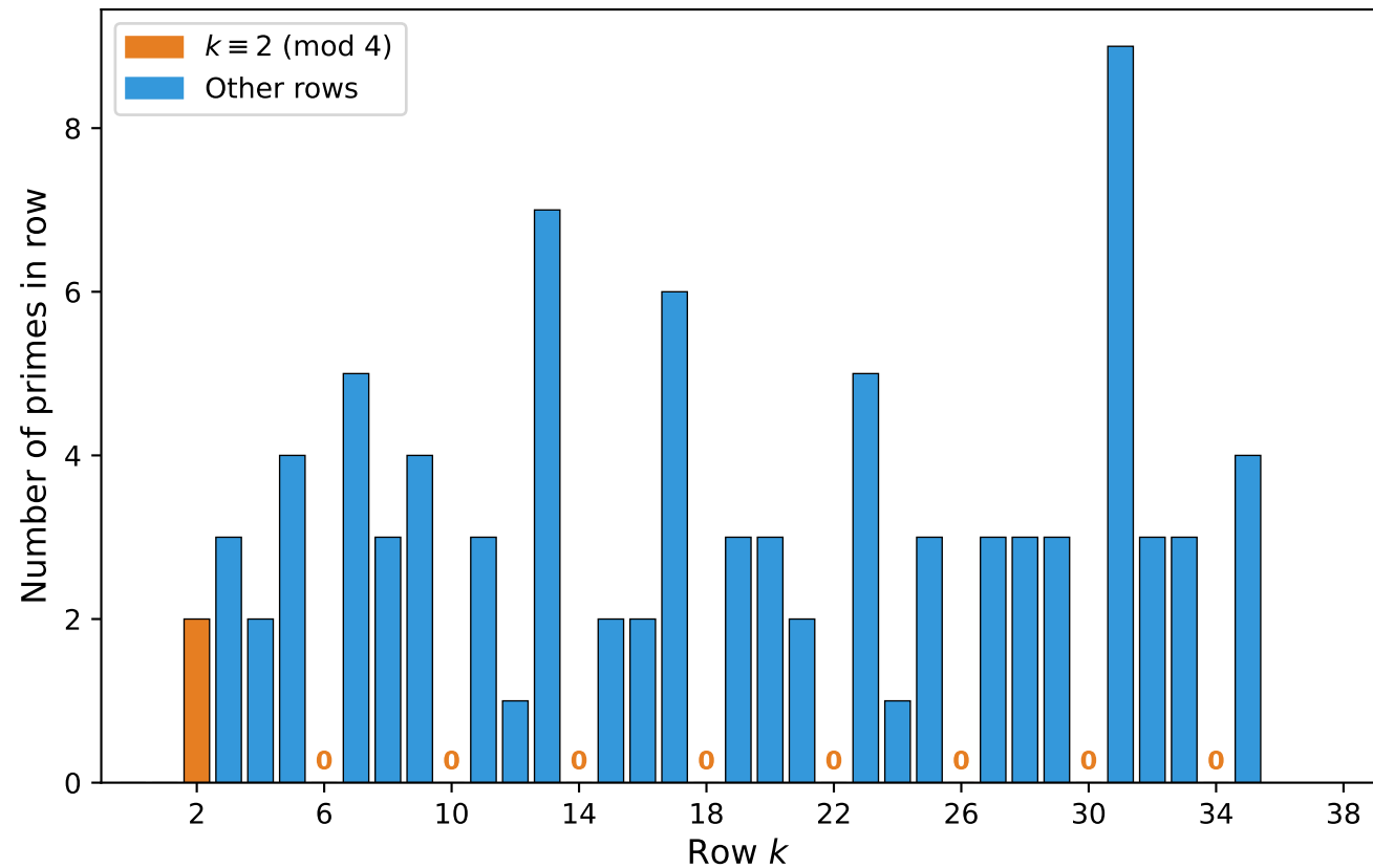
Prime counts per row in \mathcal{L}_1 (Orange: k \equiv 2 \pmod{4} , all zero for k \geq 6 )
