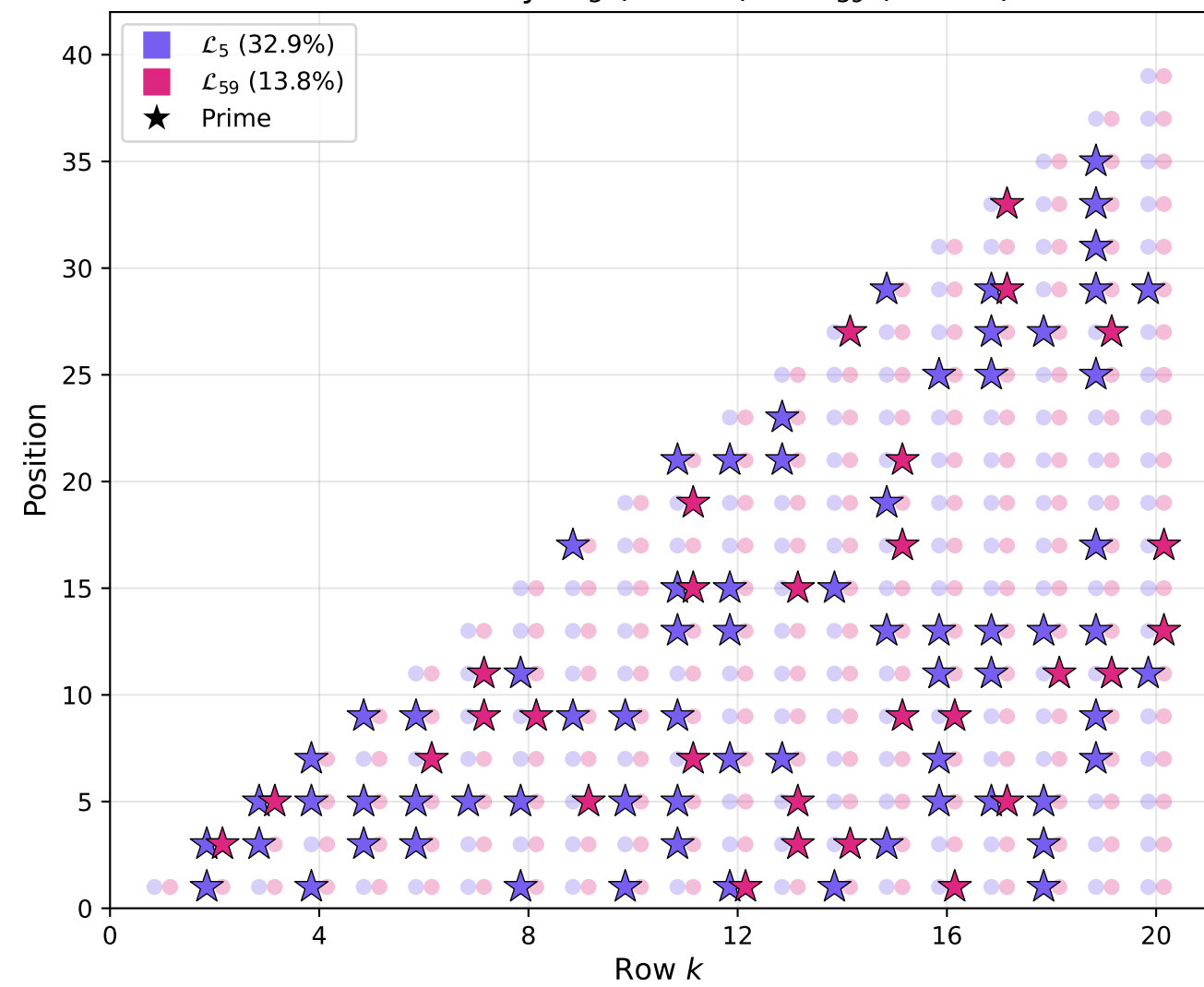
Prime density: \mathcal{L}_5 (32.9%) vs \mathcal{L}_{59} (13.8%)
