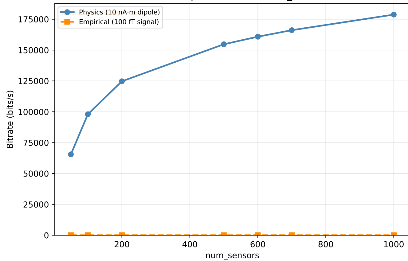
Bitrate (empirical SNR) vs num_sensors
