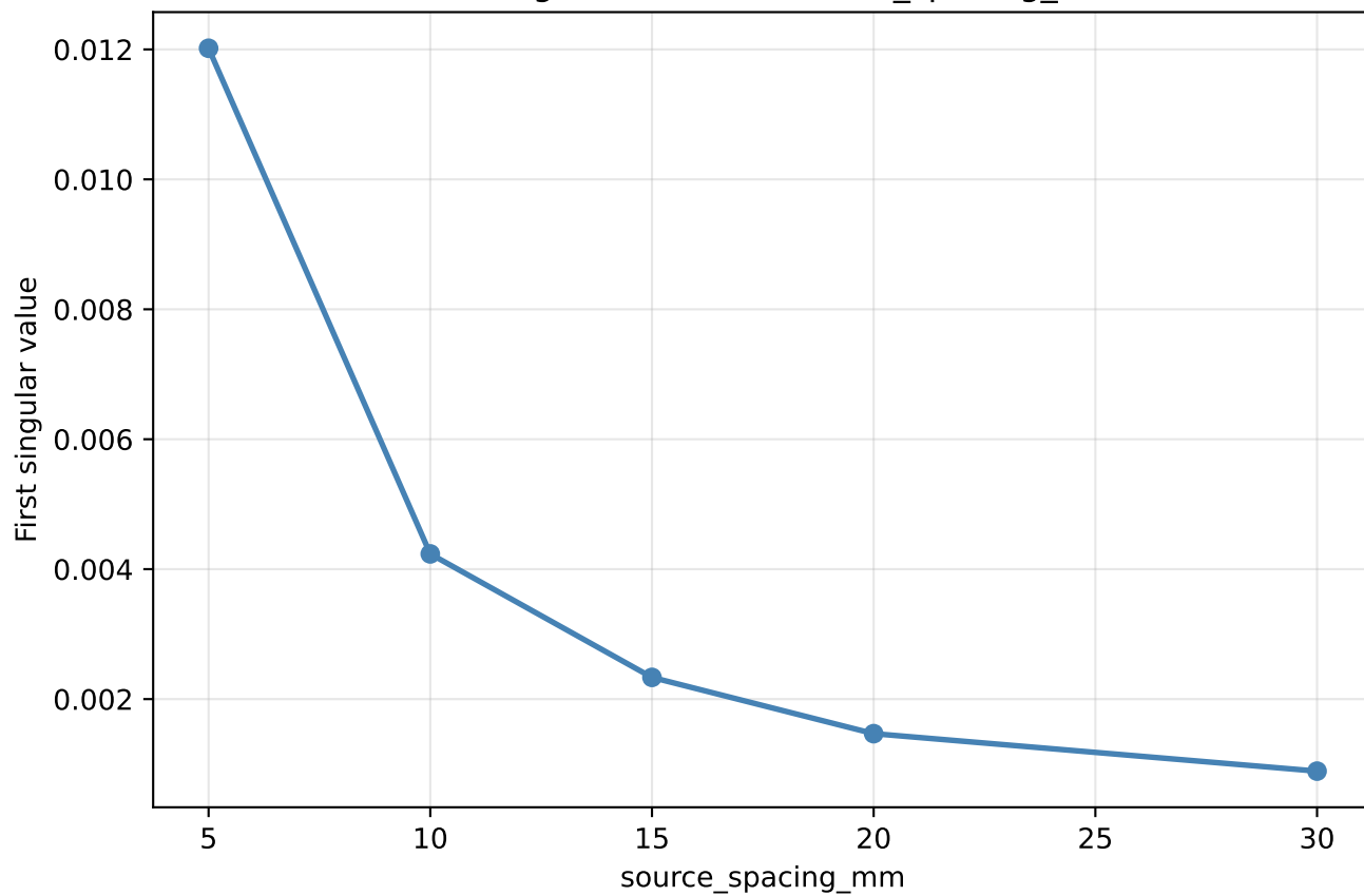
First singular value vs source_spacing_mm
