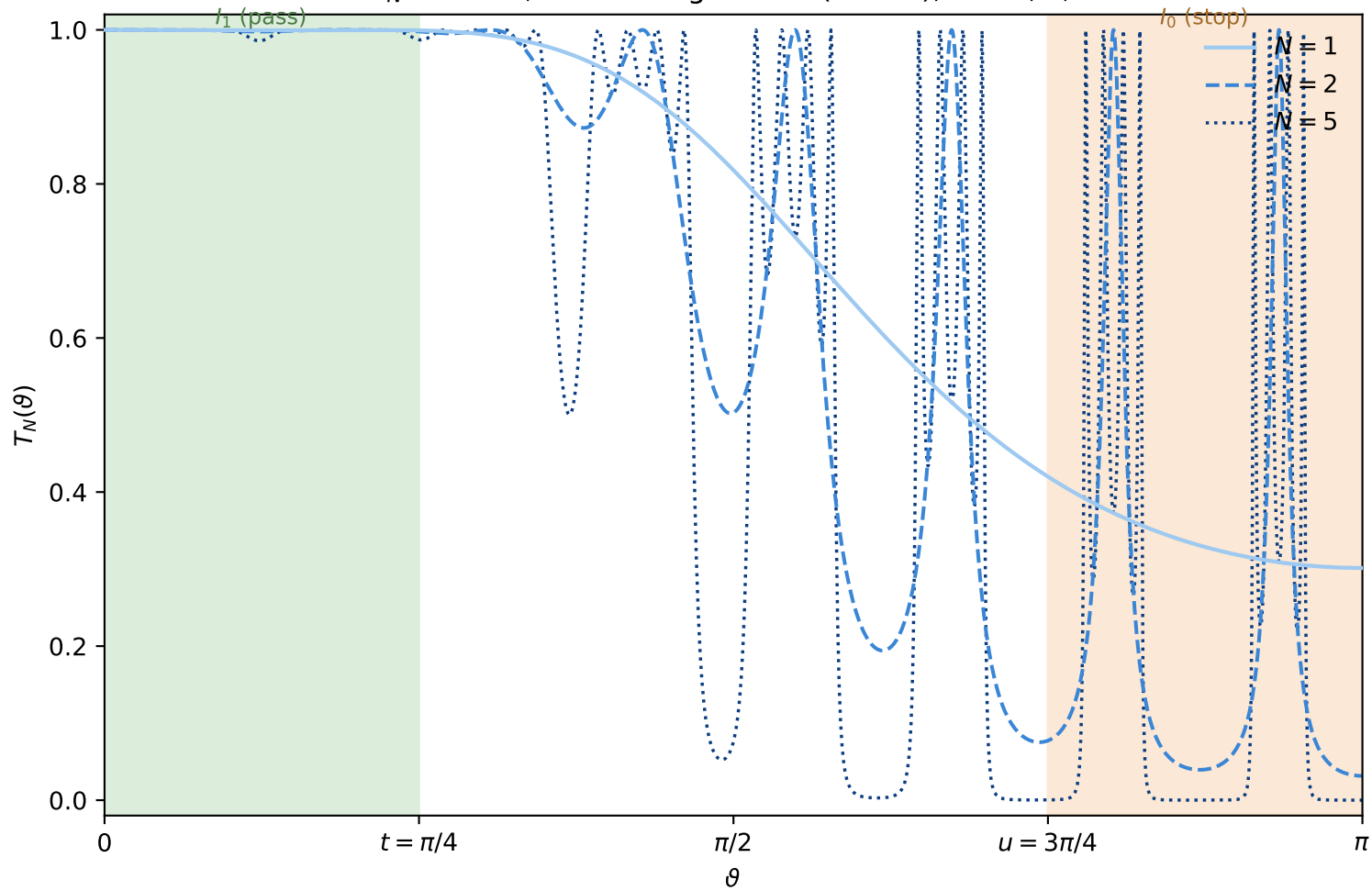
T_N at n = 3 , best configuration ( L = 16 ), N = 1, 2, 5
