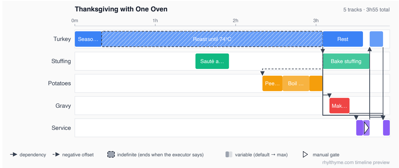
Figure 1: Thanksgiving with One Oven (five tracks, thirteen steps, 3 h 55 at planned durations) as rendered by the open-source timeline renderer ( @rhylthyme/timeline ) that also produces the MCP server’s image previews. Rows are tracks; bars are steps positioned by resolved start time. The roast is indefinite (hatched, dashed border): it ends when the cook says so, and everything downstream is planned against its default duration. Arrows are cross-track dependencies; the dashed arrow is a negative offset (peel the potatoes 45 min before the roast is due out). The flag on “Guests seated” marks a manual gate that the host fires; “Carve” waits for it, and “Serve” waits for all four dishes. The oven is a capacity-one resource, so the stuffing bakes only after the turkey comes out. The web application draws its own D3 timeline from the same JSON.
