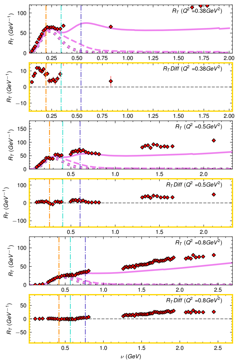
■ R_L, R_T (QE) SuSAv2 — W = 0.93 \text{ GeV} — R_T (QE+2p2h) SuSAv2 — R_L, R_T (Total) SuSAv2 — W = 1.07 \text{ GeV} ◆ R_L, R_T this - SuSAv2 ◆ R_L, R_T this analysis — W = 1.23 \text{ GeV}
