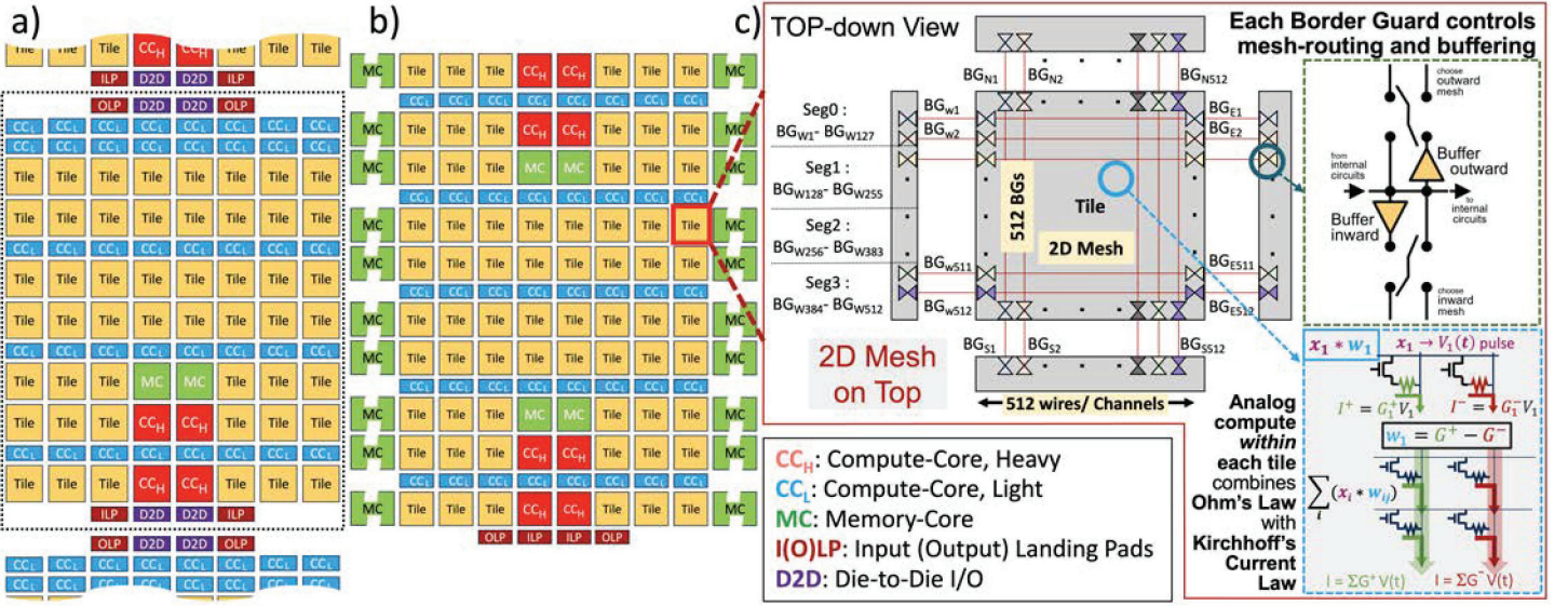
Fig. 2: A base chiplet is either a) repeated vertically to create a Fully-Weight-Stationary (FWS) system, or b) reused by weight-reloading to create a Partially-Weight-Stationary (PWS) system. Blocks such as analog-memory Tiles, Heavy and Light Compute-cores ( CC_H and CC_L ), scratchpads ( MC ), and both off-chip and Die-to-Die (D2D) IO are interconnected using c) a 2D Mesh with BorderGuard circuits (BGs) for dataflow control. In an FWS system, both Ohm's law and Kirchhoff's law allow Analog-AI compute using Non-Volatile Memory (NVM)-based resistors; in a PWS system, weight-reloading mandates high-endurance SRAM (or e-DRAM), using Kirchhoff's law or charge sharing for MAC computation with multiple word- and/or bit-lines (not shown) [8], and large Memory-Cores (or off-chip DRAM, not shown) to store layer-weights. (Part (c) adapted from [16].)
