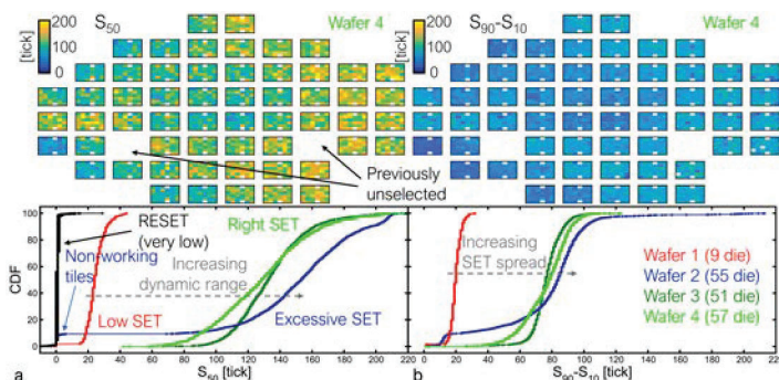
Fig.3: Full Wafer Maps and CDFs for the (a) S_{50} and (b) S_{90}-S_{10} spread, indicating the conductance change, expressed in digital integration counts, for the median (50%) SET-state conductance value and the spread between the 10% and 90% SET conductance.
