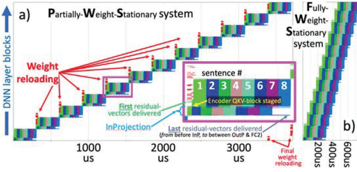
Fig.6: Progress through BERT-base DNN-layer-blocks vs. time for the (a) PWS and (b) FWS systems. The timing of the 12-layers and b=8 sentences, the staging of all sentence-tokens before initiating self-attention (QKV) compute, and the staging of residually-connected data are all visible. PWS runs include weight-reloading before a CIM-Tile can be reused with different weights, and after the workload (to return the system to its initial state).
