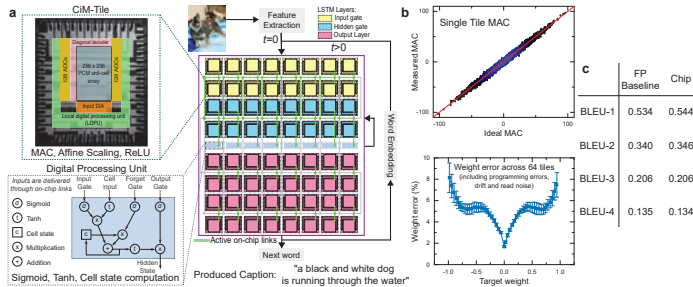
Fig. 5: a) A 64-Tile chip combines CCO-based ADCs and local digital-compute (scaling, ReLU activations) at each Tile, together with more complex digital processing (sigmoid & tanh activations, LSTM-vector OPs) at chip-center, to implement an image-captioning LSTM model. b) Highly-linear MAC operations and accurate weight-programming resulted in c) software-equivalent BLEU scores.
