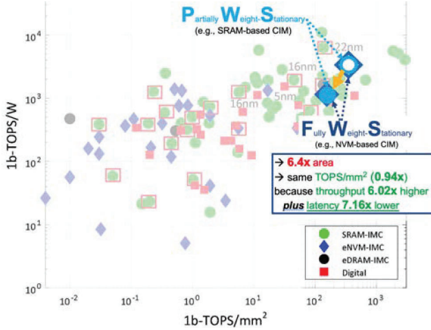
Fig. 7: 1-bit TOPS/W vs. 1-bit TOPS/sq.mm examples [8], with new data points from this study marked for Partially-Weight-Stationary (cyan solid circle) and Fully-Weight-Stationary (blue solid diamond) solutions capable of implementing BERT-large. Identical CIM-Tile performance (100 TOPS/W, 40nsec raw Tile-compute, open symbols) are assumed for PWS (e.g., SRAM-based CIM) and FWS (e.g., PCM-based CIM [16]), assuming 8-bit excitations and 4-bit (equivalent) weights.
