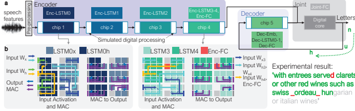
Fig. 4: (a) RNNT model transcribes input speech into words, character by character, using compute blocks mapped onto 5 chips (plus off-chip digital-compute). 45M weights are implemented with \sim 140M PCM devices, (b) with complex routing and multicasting of input- and MAC-vectors across 34 Tiles. Example sentence from experimental results, at 9.258% Word-Error-Rate [19].
