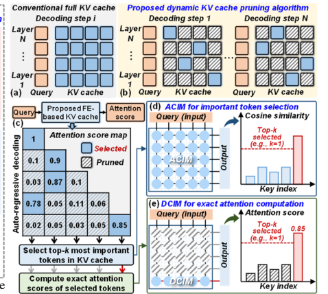
Fig. 2 (a) Conventional full KV cache. (b) Proposed dynamic KV cache pruning algorithm. (c) The framework of proposed FE-based KV cache with (d) ACIM for top-k most important token selection in KV cache and (e) DCIM for exact attention computation of a subset of selected tokens.
