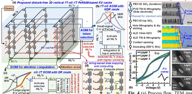
Fig. 3 (a) Proposed novel disturb-free 3D vertical 1T-nC-1T FeRAM structure for KV cache. (b) 1T-nC-based ACIM with small-signal non-destructive read (NDR) mode for token selection. (c) nC-1T DCIM with destructive read (DR) mode for attention computation. (d) Proposed nC string-based data mapping and computing schemes.
