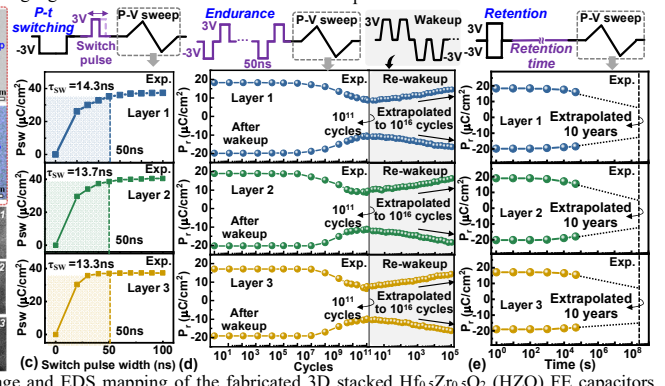
Fig. 4 (a) Process flow, TEM image and EDS mapping of the fabricated 3D stacked Hf 0.5 Zr 0.5 O 2 (HZO) Fe capacitors (FeCaps). (b) Measured P-V loops and cross-section TEM images of three-layer devices, showing excellent consistency and crystallization of FE-HZO. (c) Measured FE polarization switching characteristics of three-layer devices which can be fully switched within 50ns. (d) Measured endurance characteristics of three-layer devices under 10 11 3V 50ns pulses, and re-wakeup method is adopted after fatigue, showing extrapolated 10 16 cycles. (e) Measured retention characteristics of three-layer devices at room temperature, showing 10 years extrapolated retention time.
