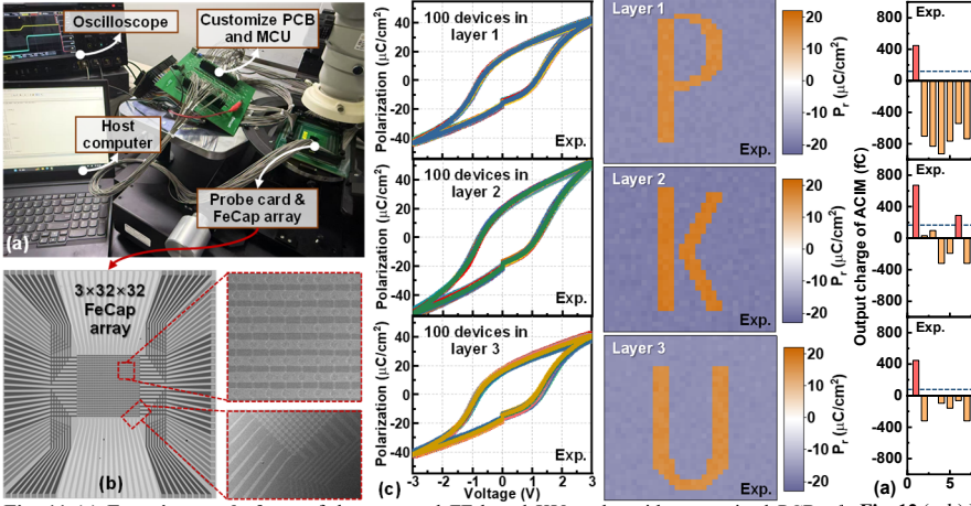
Fig. 11 (a) Experiment platform of the proposed FE-based KV cache with customized PCB of peripheral circuits and MCU. (b) Microscope image and SEM images of the fabricated 3D three-layer 3x32x32 FeCap array for storage and computation of KV cache. (c) Measured P-V curves of 100 devices in three layers and the readout pattern of three-layer devices, showing great consistency.
