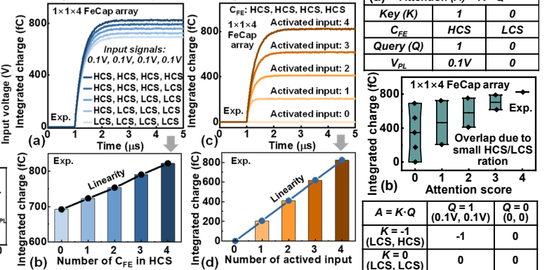
Fig. 6 (a, b) Measured integrated charges of 1x1x4 FeCap array with different stored capacitance states, showing good linearity. (c, d) Measured integrated charges of 1x1x4 FeCap array with different activated inputs, also showing good linearity.
