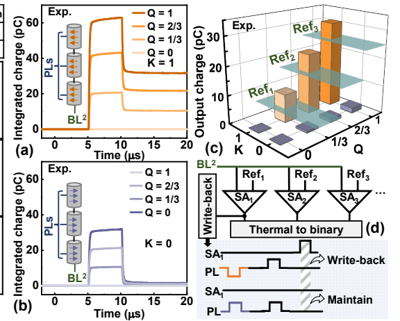
Fig. 10 Measured integrated charges of three-layer FeCaps written to (a) -P r (key of 1) and (b) -P r (key of 0) state with different input signals on plate-lines (PLs) for different query. (c) Measured compute results indicating the similarity between query and key, showing great linearity. (d) Proposed multi-bit sense amplifier (MBSA) design with write-back.
