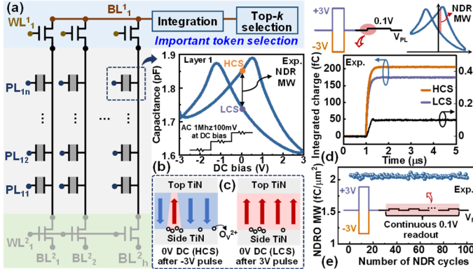
Fig. 5 (a) Schematic of proposed 1T-nC-based ACIM. (b) Measured asymmetric small-signal C-V of first-layer FeCap, showing NDR memory window (MW) at DC 0V, caused by (c) oxygen vacancies at the side TiN electrode. (d) Measured capacitive NDR MW by integrating current flowing onto the FeCap. (e) Measured one hundred repeated NDR cycles.
