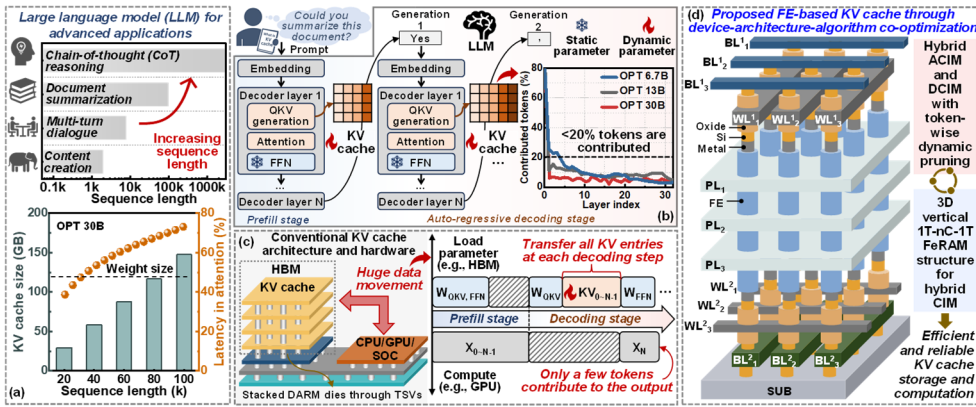
Fig. 1 (a) Large language models (LLMs) for advanced applications with increasing sequence length, and the impact of sequence length on key-value (KV) cache size and attention latency. (b) The workflow of transformer-based generative AI application, where the KV cache is dynamically generated and only a small subset of tokens are contributed, exhibiting significant sparsity. (c) Conventional KV cache architecture and hardware with huge data movement, along with the limited capacity and high bit cost of HBM, constrained by the die stacking technology. (d) Proposed 3D 1T-nC-1T ferroelectric (FE)-based KV cache featuring hybrid analog compute-in-memory (ACIM) and digital CIM (DCIM) architecture with token-wise dynamic pruning algorithm.
