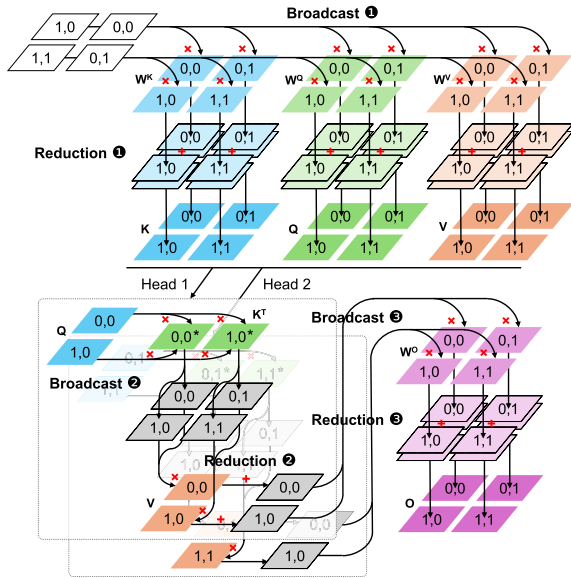
Fig. 7. Collective communication overhead incurred by tiling and unrolling key MM in an example layer of the original attention. Note that the nonlinear operations are not included in this illustration.
