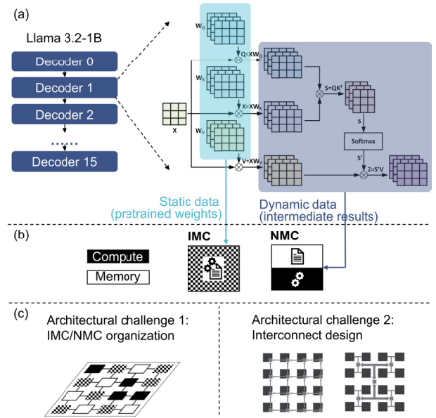
Fig. 1. (a) The basic LLM structure, (b) the data stationarity-based MM assignment on the IMC/NMC system, and (c) the primary challenges in hybrid IMC/NMC system design.
