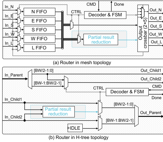
Fig. 9. Router architecture with partial result reduction in (a) mesh and (b) H-tree topology interconnected cores.
