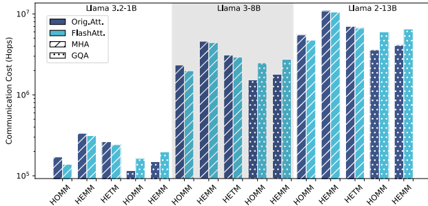
Fig. 12. Communication overhead of LLM inference under various architectural organizations and attention mechanisms.
