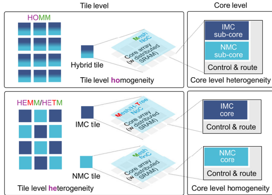
Fig. 2. The hardware hierarchy and the categorization of homogeneity and heterogeneity. Note that the placement of the IMC tiles and the NMC tiles in HE architecture is not fixed. The chessboard placement in the above figure is a toy example.
