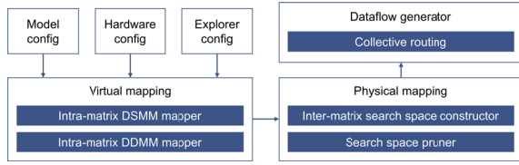
Fig. 3. JADE orchestration framework covers three key parts: virtual mapping, physical mapping, and dataflow routing.
