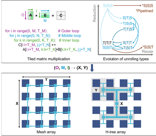
Fig. 4. Large MM tiling and spatial unrolling on 2D hardware arrays with mesh or H-tree topologies.
