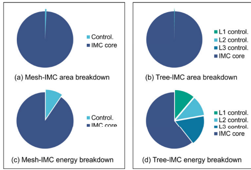
Fig. 10. Area and energy breakdown of the IMC cores in mesh and H-tree topologies. L1, L2, and L3 refer to different levels of routers in the H-tree interconnection.
