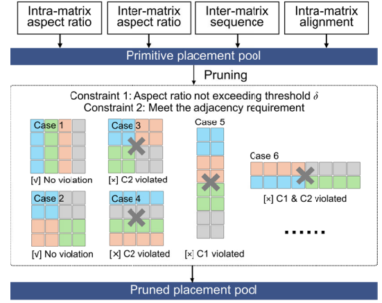
Fig. 5. Inter-matrix mapping design space generation and pruning for mesh topologies.
