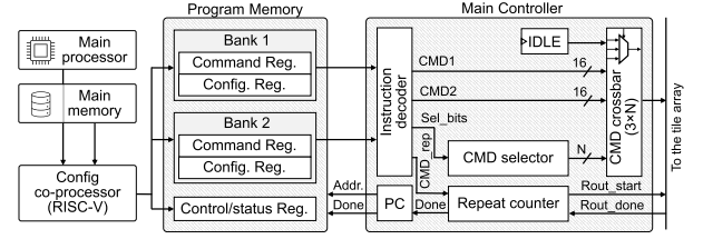
Fig. 8. The system-level architecture of JADE includes program memory, main controller, and the tile array.
