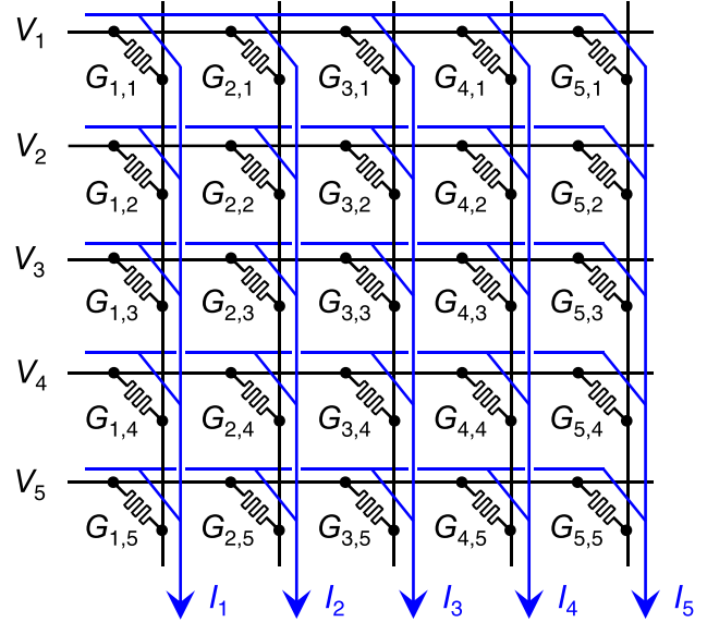
FIG. 5. The basic concept of a massively parallel analog vector-matrix multiplication within a resistive memory crossbar. The currents accumulated by the columns are given by Eq. (5).
