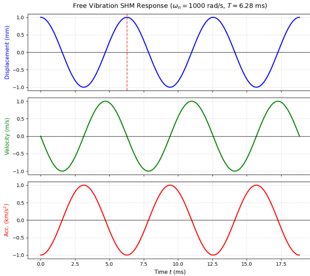
Fig. 12: Position, velocity and Acceleration of the System
