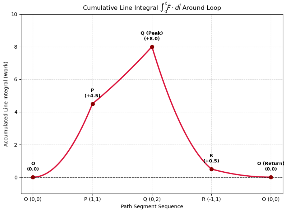
Fig. 5: Cancellation of Integrals Plotted
