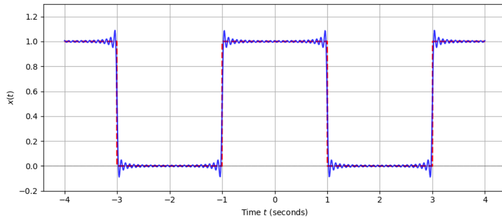
Fig. 7: Gibb's Phenomenon Plotted
