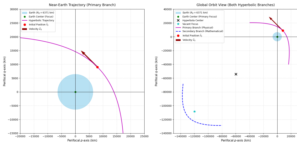
Fig. 1.2.8.1 Trajectory of the Satellite
