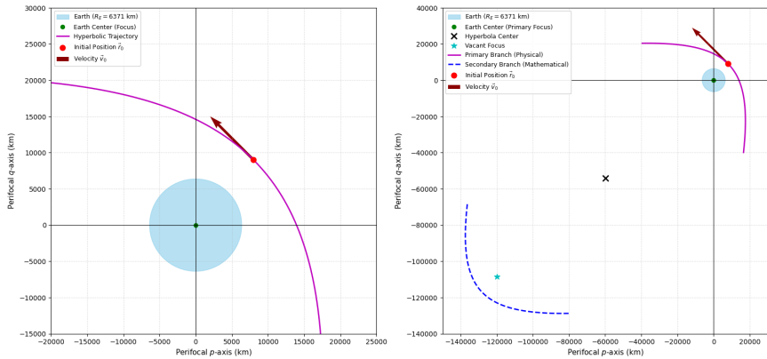
Fig. 1.2.40.1: Trajectory of satellite
