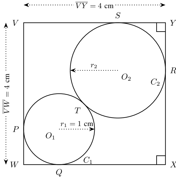
Fig. 1.2.37.2
