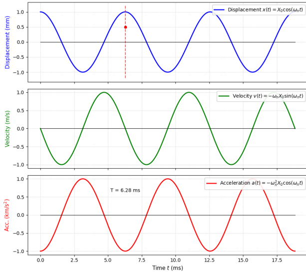
Fig. 1.2.39.1: Acceleration, Velocity and Position of the System
