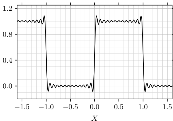
Fig. 1.2.37.6: Gibbs phenomenon
