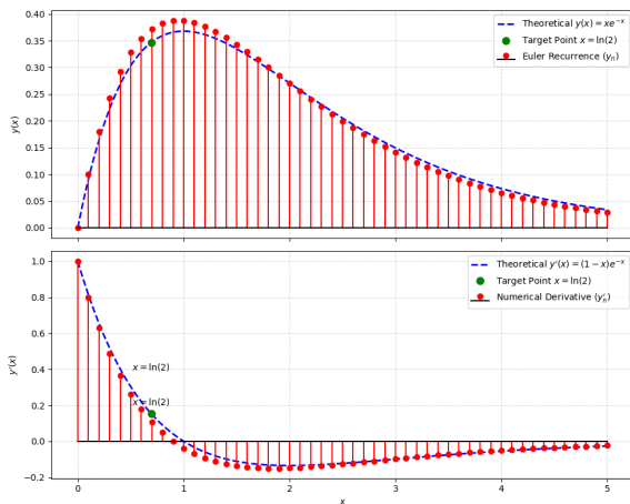
Fig. 1.2.37.7: (1.2.37.39) vs (1.2.37.43)
