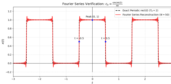
Fig. 1.1.18.1: Gibbs phenomenon
