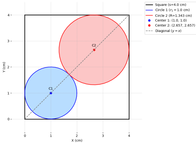
Fig. 1.2.37.3: Square with Tangent Circles
