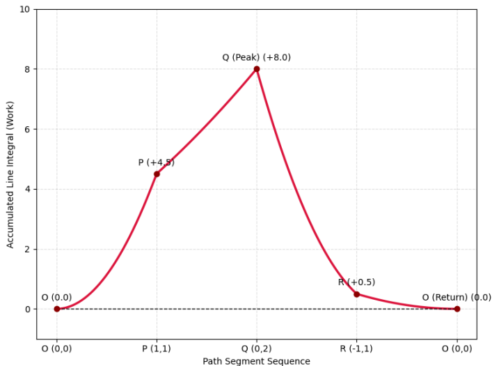
Fig. 1.2.37.5
