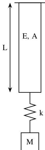
Fig. 1.1.35.1: Spring mass system
