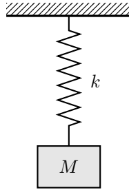
Fig. 1.1.28.1: Spring Mass system in vertical plane
