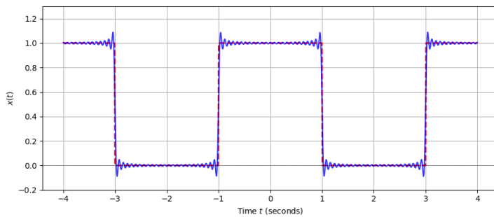
Fig. 7.2 Gibb's Phenomenon
