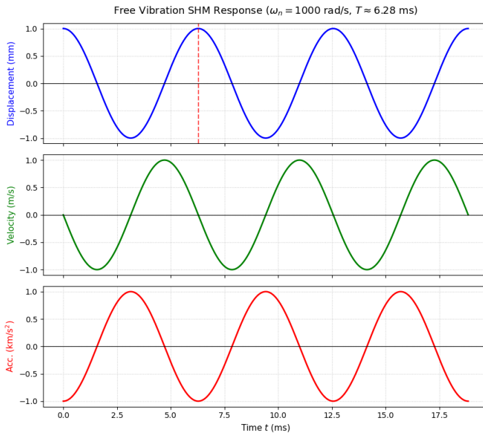
Fig. 16.2 Acceleration, Velocity and Position of the System
