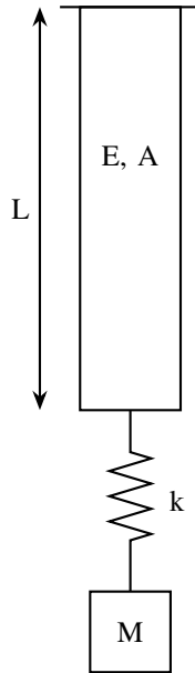
Fig. 16.1 Diagram of the system
