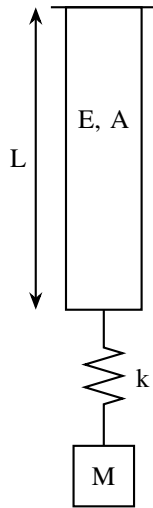
Fig. 1.2.13.1 Diagram of the system
