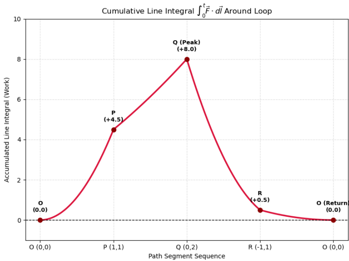
Fig. 1.2.5.2 Visualising the Cancellation of Integrals
