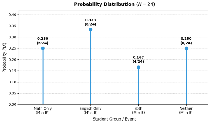
Fig. 1.2.2.1 Probability Distribution
