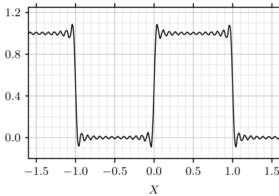
Fig. 1.2.6.1 Fourier Square Wave Representation
