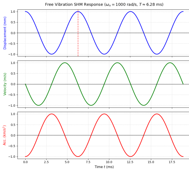
Fig. 1.2.13.2 Acceleration, Velocity and Position of the System
