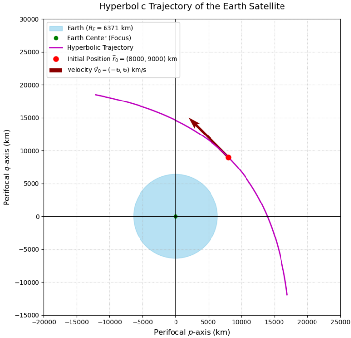
Fig. 1.2.9.1 Trajectory of the Satellite
