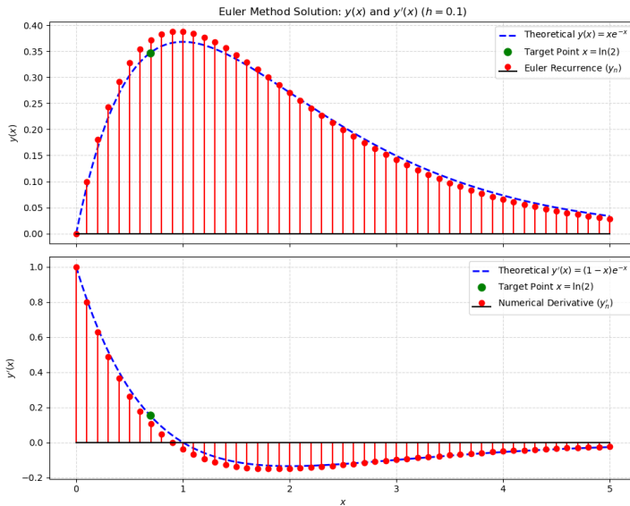
Fig. 1.2.11.1 Theoretical Plot vs Plot obtained with Euler's Forward Difference Method
