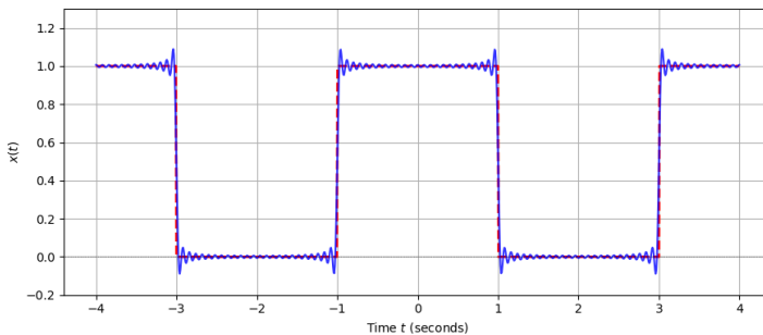
Fig. 1.2.6.2 Gibbs Phenomenon
