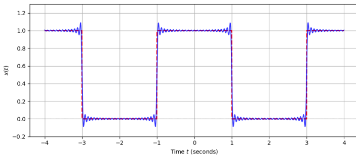
Fig. 7.2 Gibbs Phenomenon
