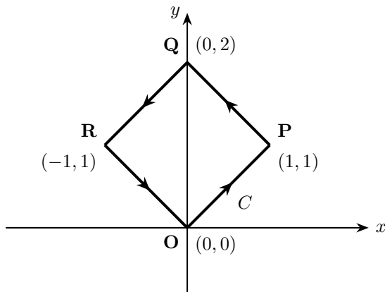
Fig. 1.2.38.4: Contour C
