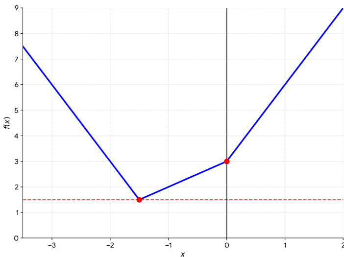
Fig. 1.2.39.1: Plot of the function
