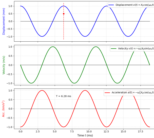
Fig. 1.2.40.1: Acceleration, Velocity and Position of the System
