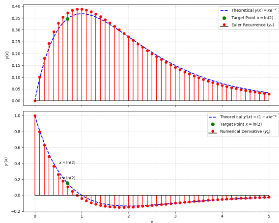
Fig. 1.2.38.7: (1.2.38.39) vs (1.2.38.43)
