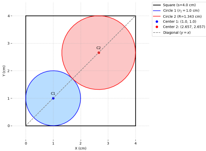
Fig. 1.2.38.3: Square with Tangent Circles
