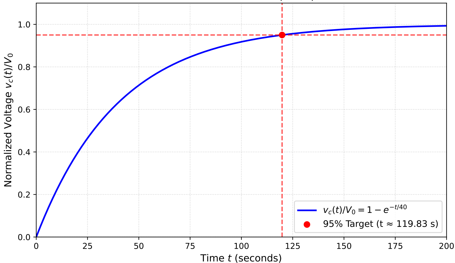
RC Circuit First-Order Step Response
