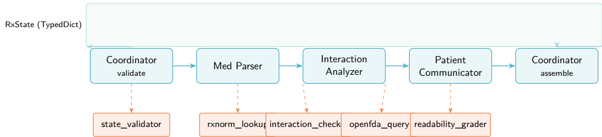
Figure 1: High-level architecture. Solid arrows show state flow; dashed arrows show tool invocations. The shared RxState TypedDict is threaded through every node.
