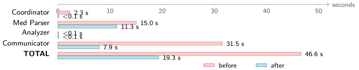
Figure 4: Per-agent latency before and after performance tuning. Median pipeline time on Apple M2 (8 GB RAM) running qwen2.5:3b .
