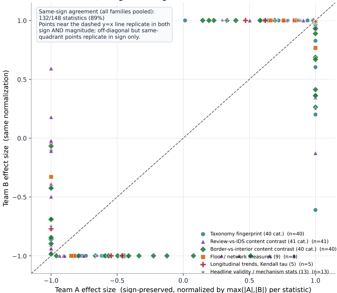
Figure 11. n = 148 headline statistics spanning validity checks, content-taxonomy profiles, floor-structure measures, and longitudinal trends, each computed independently in Team A and Team B using identical methods (Studies 1-10). Values are normalized per statistic (divide both teams' estimates by whichever is larger in magnitude, preserving sign), so the y=x line represents perfect cross-team replication and quadrant membership (top-right / bottom-left vs. top-left / bottom-right) directly shows sign agreement. One explicitly flagged sign non-replication (facilitator-share longitudinal trend) sits in an off-diagonal quadrant; a second flagged non-replication (initiator-rank stability) agrees in sign but differs sharply in magnitude, among the gray stars/plus markers.
